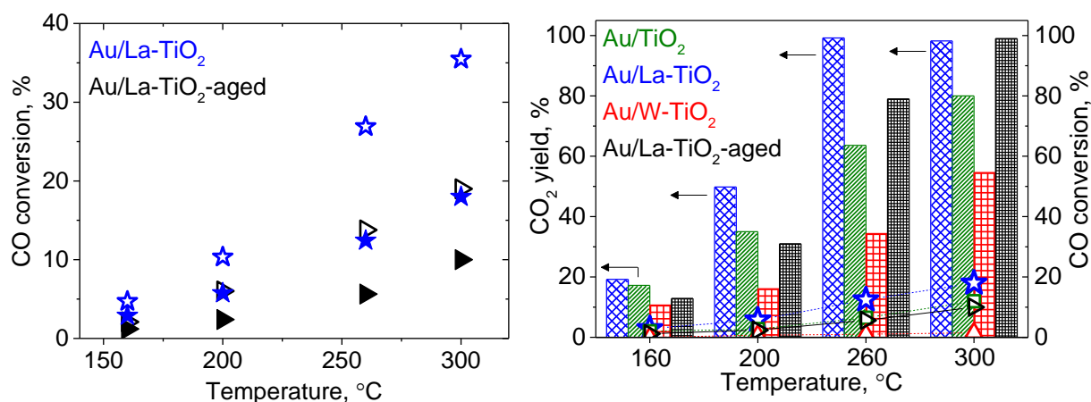
Figure 5.6 Oxidation of 650 ppm carbon monoxide (gas-phase) over Au/La-TiO 2 and Au/La-TiO 2 -aged in the presence (closed symbols) and absence of water (open symbols) (left) and comparison of carbon dioxide produced from formic acid decomposition (bars) and gas-phase carbon monoxide oxidation (scatters) as a function of temperature over Au/TiO 2 , Au/W-TiO 2 , Au/La-TiO 2 and Au/La-TiO 2 -aged catalysts using 650 ppm formic acid and 650 ppm carbon monoxide at W/F = 1.6 \times 10^{-4} \text{ g s cm}^{-3} (right).
