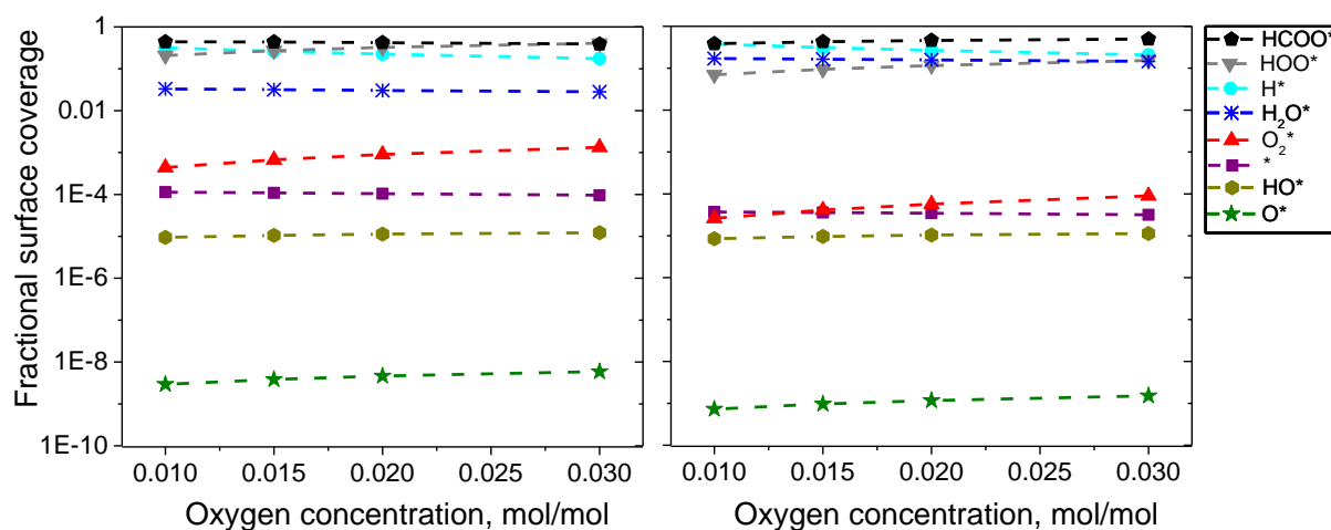
Figure 7.9 Predicted surface coverages as a function of oxygen concentration (Case III, Table 7.1) at 300 °C (left) and 200 °C (right).
