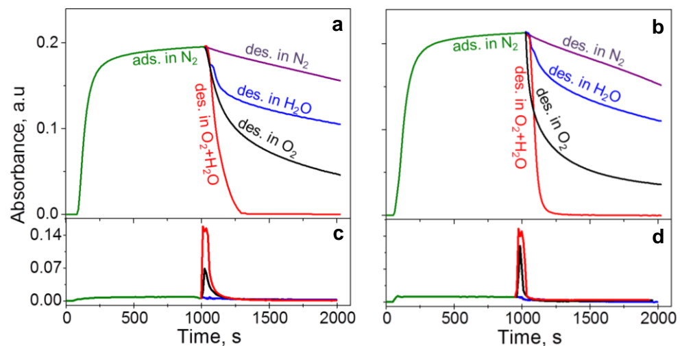
Figure 6.7 Temporal evolution of the C-H vibrational mode of formate at 2873 cm -1 on Au/La-TiO 2 at (a) 200 and (b) 260 °C during formic acid adsorption in the indicated feed. (c, d) Corresponding carbon dioxide trace from gas phase FTIR analysis.
