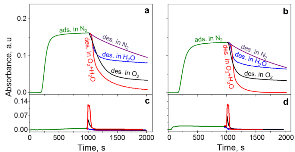
Figure 6.8 Temporal evolution of the C-H stretch vibrational mode of formate at 2873 cm -1 on Au/TiO 2 at (a) 200 and (b) 260 °C during formic acid adsorption in the indicated feed. (c, d) Corresponding carbon dioxide trace from gas phase FTIR analysis.
