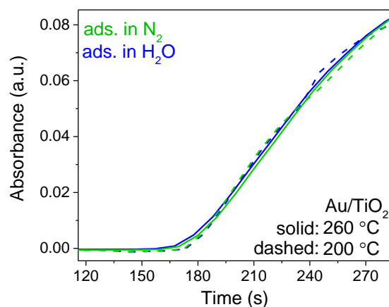
Figure 6.6 Temporal evolution of the C-H stretch vibrational mode of formate at 2873\text{ cm}^{-1} on \text{Au/TiO}_2 at 200 and 260 °C during formic acid adsorption in the indicated feed.
