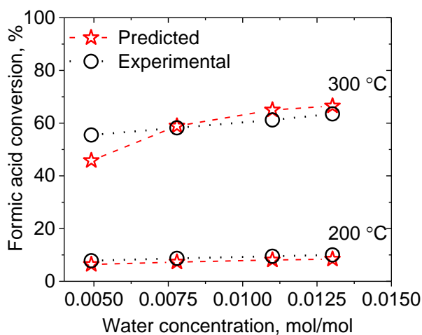
Figure 7.10 Simulated and measured trends in formic acid conversion as a function of water concentration (Case IV, Table 7.1) at 200 °C and 300 °C.
