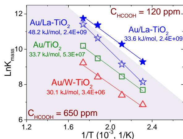
Figure 5.8 Arrhenius plots for Au/TiO 2 , Au/W-TiO 2 and Au/La-TiO 2 for formic acid decomposition at W/F = 2.4 \times 10^{-5} g s cm -3 .
