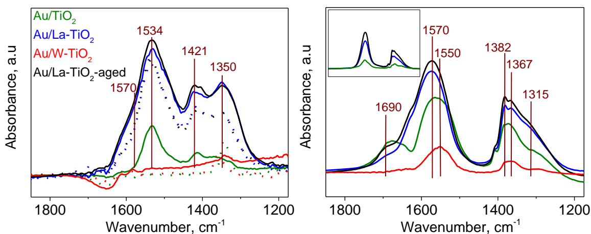
Figure 5.2 In situ DRIFT spectra of 1000 ppm carbon dioxide adsorbed on Au/TiO 2 , Au/La-TiO 2 , Au/W-TiO 2 and Au/La-TiO 2 -aged and their corresponding supports (dotted spectra) at 200°C (left) and 1120 ppm formic acid adsorbed on Au/TiO 2 , Au/La-TiO 2 , Au/W-TiO 2 and Au/La-TiO 2 -aged at 200°C (right). Inset: In situ DRIFT spectra in the presence of 10% oxygen and 5% water in the same energy range (proportional XY scales).
