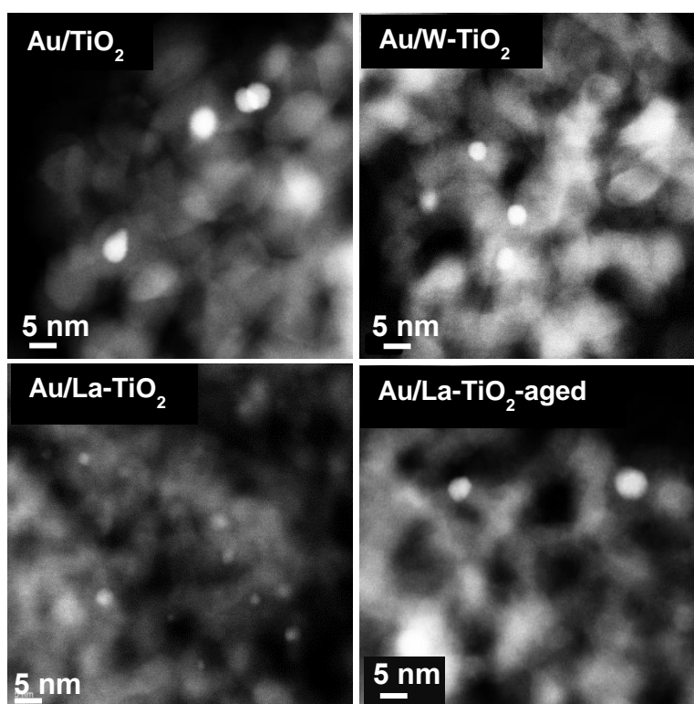
Figure 5.3 HAADF-STEM images of Au/TiO 2 , Au/W-TiO 2 , Au/La-TiO 2 and Au/La-TiO 2 -aged catalysts.
