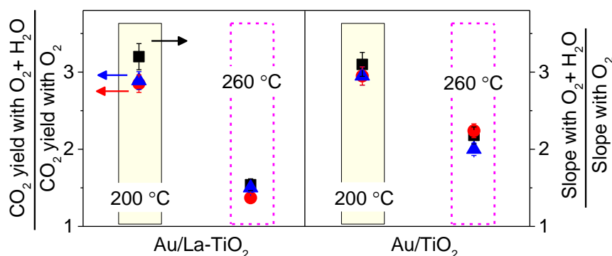
Figure 6.10 Relative yields of the carbon dioxide produced from formic acid decomposition on Au/La-TiO 2 and Au/TiO 2 in oxygen-water mixture and only oxygen derived from the catalytic experiments (▲), the ratio of slopes of the decrease in the C-H signal ( 2873\text{ cm}^{-1} ) from transient DRIFTS experiments (■) and ratio of carbon dioxide peak areas obtained from formic acid decomposition in oxygen-water mixture to that in only oxygen derived from the gas phase FTIR analysis (●).
