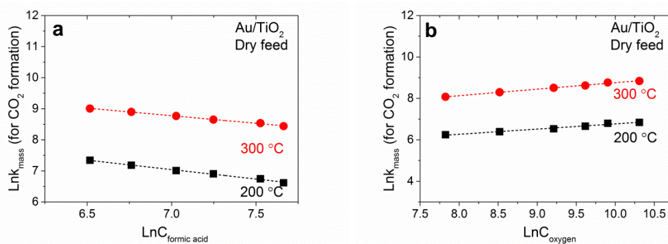
Figure 6.17 Plots used to calculate the apparent reaction orders at 200 °C and 300 °C for \text{CO}_2 formation from formic acid decomposition on \text{Au/TiO}_2 in dry feed by varying (a) formic acid concentration in the range 700-2,200 ppm and (b) oxygen concentration in the range 2500-30,000 ppm.
