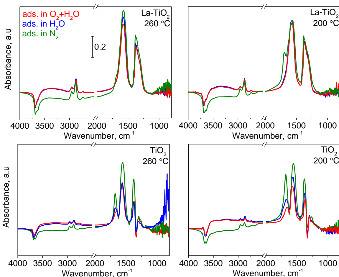
Figure 6.4 DRIFT spectra of formic acid adsorption on La-TiO 2 and TiO 2 obtained under different feed conditions at 200 °C and 260 °C.
