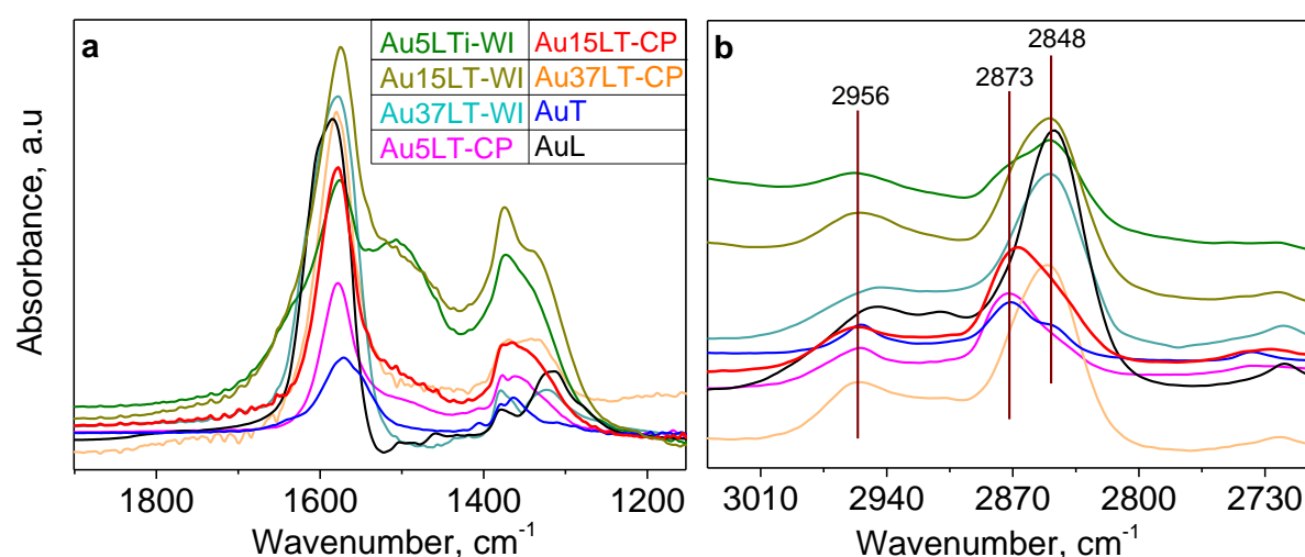
Figure 8.6 In situ DRIFT spectra of formic acid adsorption on selected gold catalysts at 260°C. Conditions: 1120 ppm formic acid, 10 vol% oxygen and 5 vol% water. Spectral range showing the carboxyl and C-H bands of formates are presented in (a) and (b), respectively.
