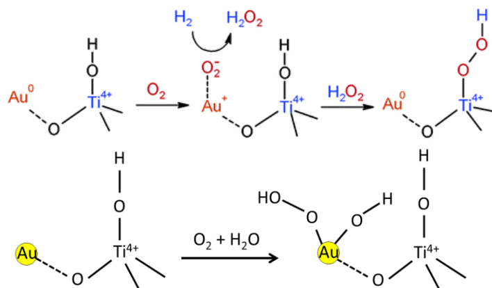
Figure 9.1 Proposed mechanistic model for the formation of hydroperoxy species on gold supported on titanasilicate from oxygen and hydrogen (top) or water (bottom). Top figure adapted with permission from Reference [294] . Copyright 2006 American Chemical Society. Bottom figure adapted with permission from Reference [128] . Copyright 2009 John Wiley and Sons.
