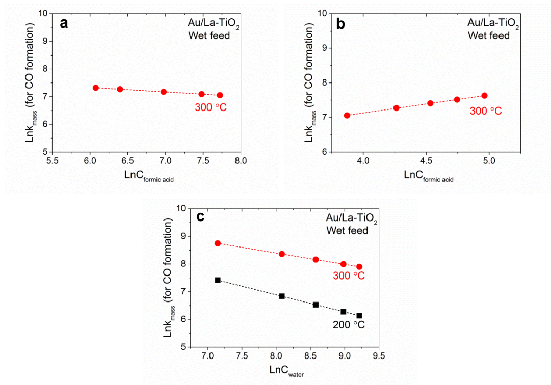
Figure 6.14 Plots used to calculate the apparent reaction orders at 200 °C and 300 °C for CO formation from formic acid decomposition on Au/La-TiO 2 in wet feed by varying (a-b) formic acid concentration in the range 400-2,200 ppm and 50-150 ppm, respectively and (c) water concentration in the range 1000-10,000 ppm.
