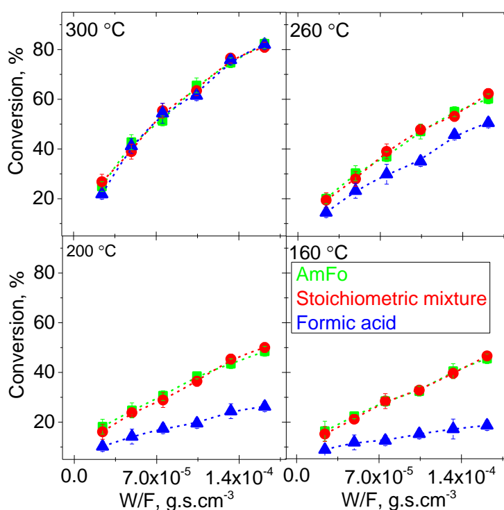
Figure 4.1 Kinetic traces depicting formic acid conversion as a function of contact time, expressed as W/F ( \text{g cat s cm}^{-3} ) obtained over 0.5 wt% Au/TiO 2 by using AmFo, formic acid and stoichiometric ammonia-formic acid mixture at different temperatures.
