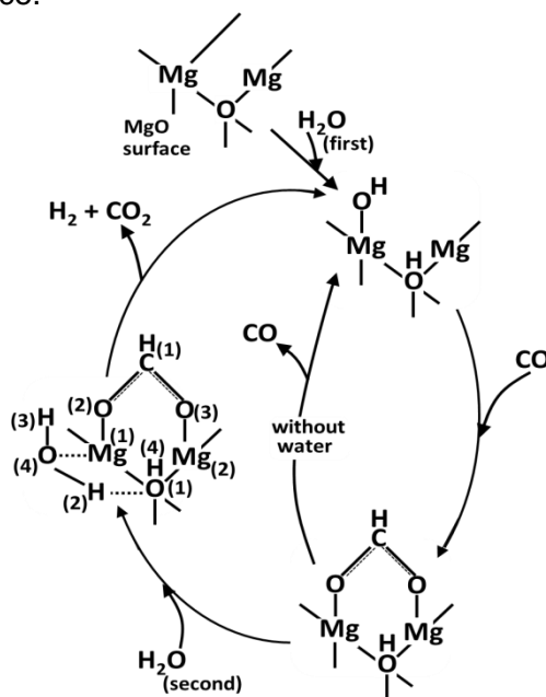
Figure 1.3 Proposed mechanism for WGS on magnesium oxide. Adapted from Reference [54] , Copyright (1990), with permission from Elsevier.
