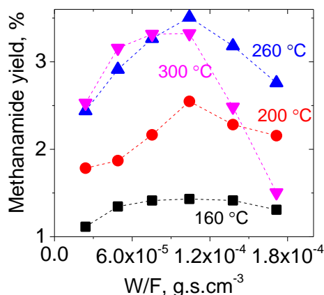
Figure 4.4 Evolution of methanamide yield as a function of contact time at different temperatures during AmFo decomposition over 0.5 wt% Au/TiO 2 .
