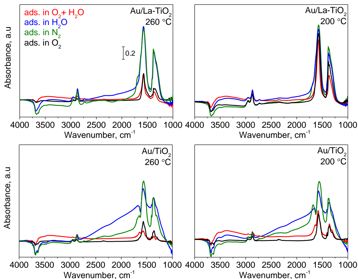
Figure 6.5 Steady state DRIFT spectra of formic acid adsorption on Au/La-TiO 2 and Au/TiO 2 obtained under different feed conditions at 200 °C and 260 °C.
