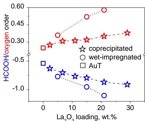
Figure 8.11 Influence of lanthana content in the gold catalysts prepared by coprecipitation and wet-impregnation on reaction orders in formic acid and oxygen at 300 °C.
