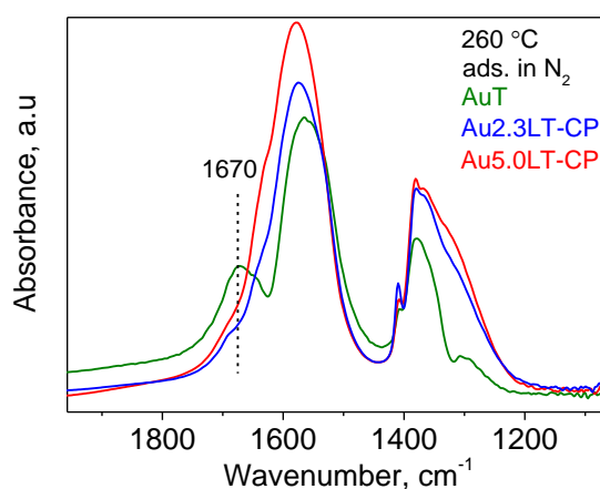
Figure 8.14 In situ DRIFTS spectra of formic acid adsorption in nitrogen on gold catalysts of different lanthana loadings showing the inhibition of the band at 1670 cm -1 .
