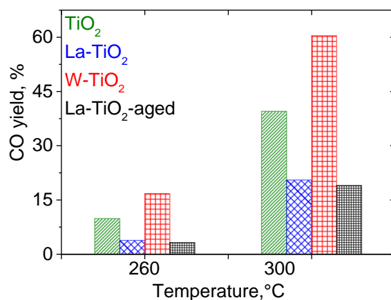
Figure 5.9 Comparison of carbon monoxide yield from formic acid decomposition on titania, tungsten-modified titania and fresh and aged lanthanum-modified titania at \text{W/F} = 1.6 \times 10^{-4} \text{ g s cm}^{-3} .
