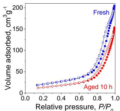
Figure 3.2 Nitrogen sorption isotherms of fresh and 10 h hydrothermally aged 0.5 wt% Au/TiO 2 catalysts. Closed symbols indicate the adsorption branch while the open symbols represent the desorption branch.
