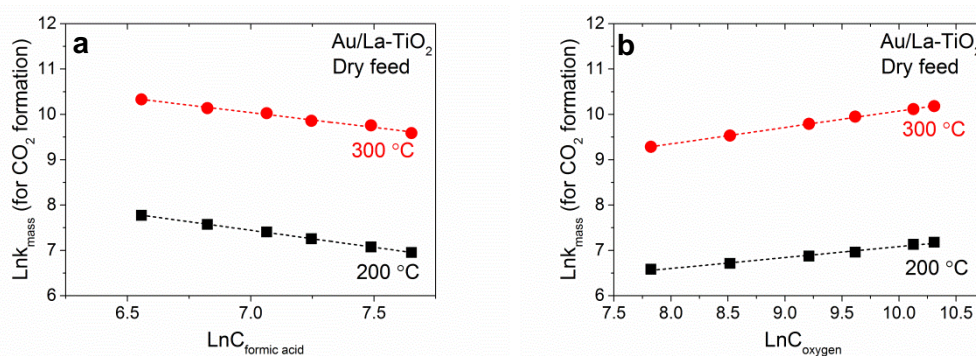
Figure 6.13 Plots used to calculate the apparent reaction orders at 200 °C and 300 °C for \text{CO}_2 formation from formic acid decomposition on Au/La-TiO 2 in dry feed by varying (a) formic acid concentration in the range 700-2,200 ppm and (b) oxygen concentration in the range 2500-30,000 ppm.
