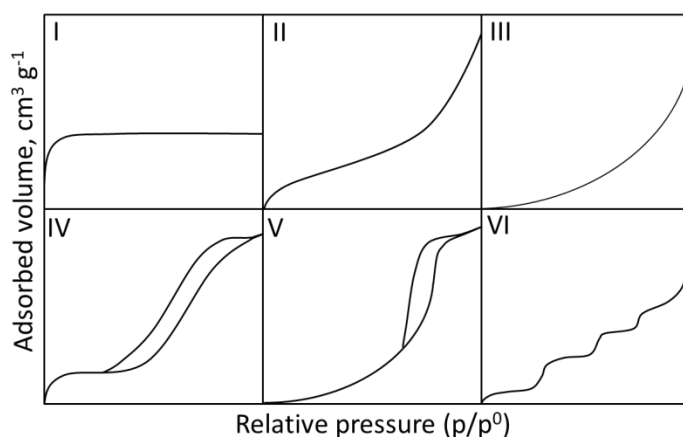
Figure 2.1 BET N 2 -adsorption isotherms
