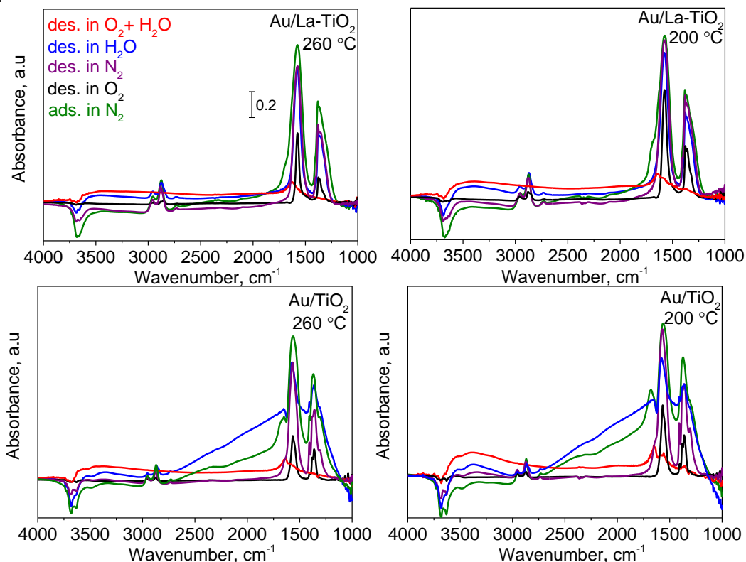
Figure 6.9 DRIFTS spectra of formic acid adsorption in nitrogen and desorption in nitrogen, oxygen, water and oxygen-water mixture on Au/TiO 2 and Au/La-TiO 2 at 200\text{ }^{\circ}\text{C} and 260\text{ }^{\circ}\text{C} .
