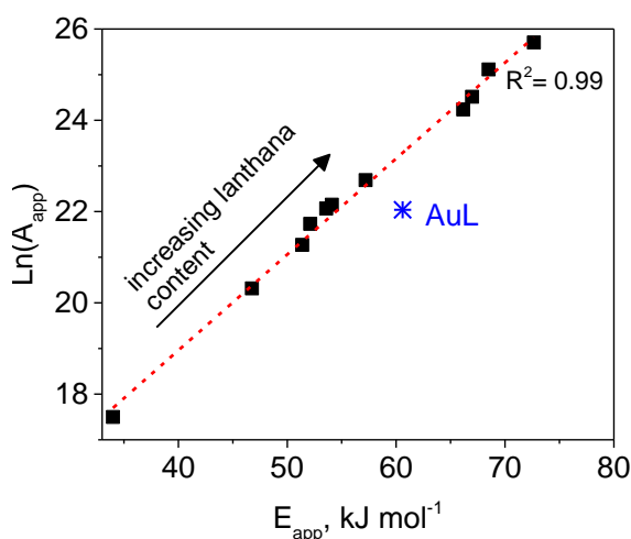
Figure 8.12 Constable plot of pre-exponential factor ( A_{app} ) and the apparent activation energy ( E_{app} ) for formic acid decomposition over gold catalysts prepared by coprecipitation.
