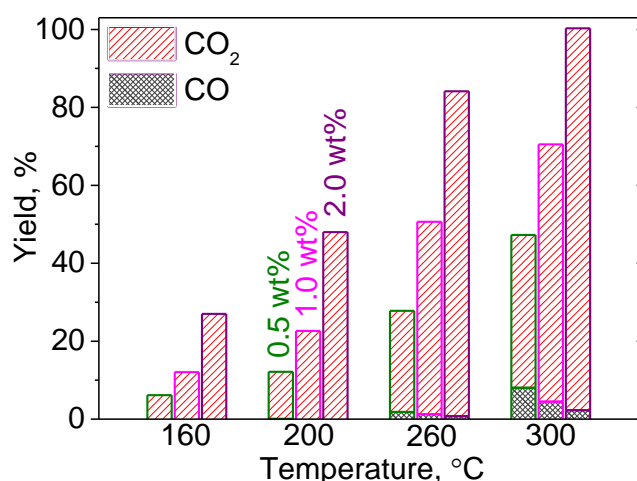
Figure 5.10 Effect of gold loading on the product distribution during formic acid decomposition over the unmodified support as a function of temperature at W/F = 4.9 \times 10^{-5} \text{ g s cm}^{-3} .
