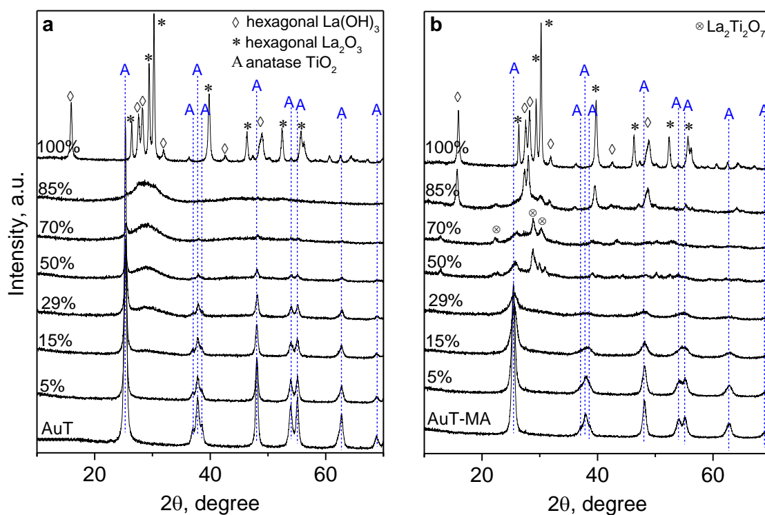
Figure 8.1 XRD patterns of the lanthanum-modified catalysts prepared by (a) wet-impregnation and (b) coprecipitation.
