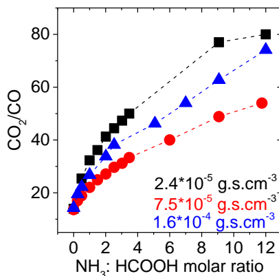
Figure 4.8 Molar ratio of reaction products, namely, carbon dioxide and carbon monoxide as a function of ammonia to formic acid molar ratio.
