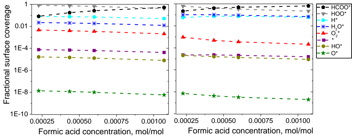
Figure 7.7 Predicted surface coverages as a function of formic acid concentration (Case II, Table 7.1) at 300 °C (left) and 200 °C (right).
