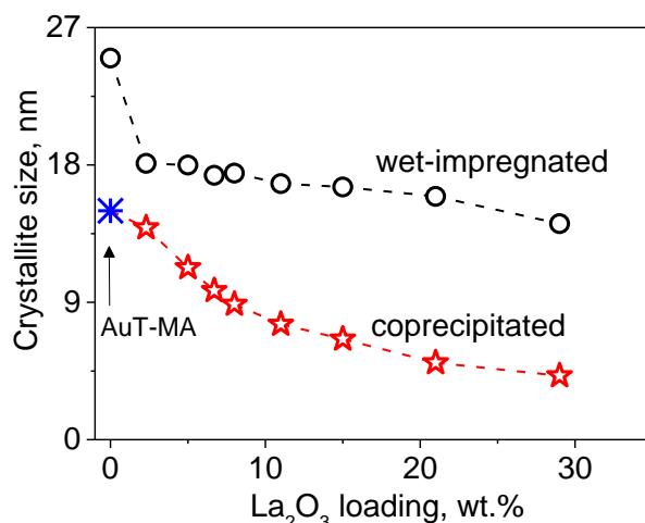
Figure 8.3 Crystallite size (nm) as a function of lanthana loading in gold catalysts prepared by coprecipitation and wet impregnation. The blue star represents AuT-MA.
