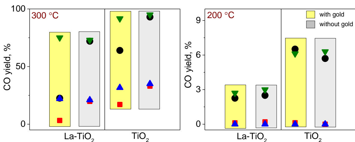
Figure 6.3 Comparison of carbon monoxide yield obtained from decomposition of 750 ppm formic acid over \text{Au/La-TiO}_2 , \text{Au/TiO}_2 and the corresponding supports at 200 °C and 300 °C using different feed compositions: nitrogen (▼), 10 vol % oxygen (●), 5 vol% water (▲) and mixture of 10 vol% oxygen and 5 vol % water (■) at W/F = 1.6 \times 10^{-4} \text{ g s cm}^{-3} .
