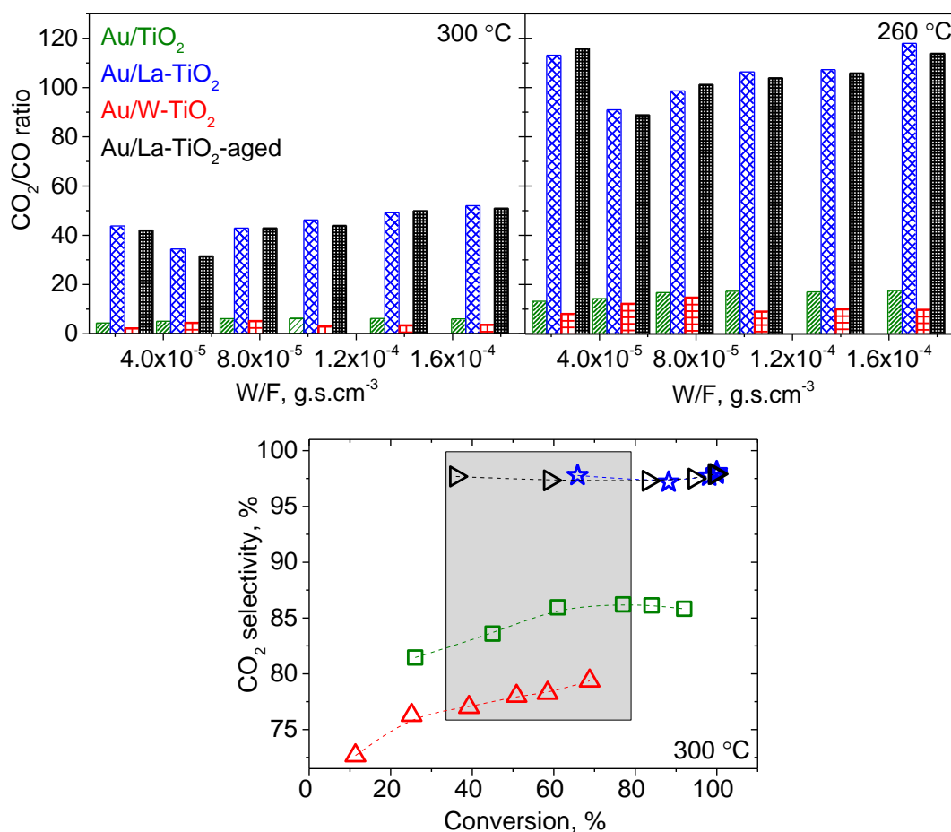
Figure 5.5 Evolution of CO 2 /CO ratio as a function of contact time obtained from formic acid decomposition over Au/TiO 2 , Au/W-TiO 2 , Au/La-TiO 2 and Au/La-TiO 2 -aged catalysts at 300 °C and 260 °C ( top) and formic acid conversion versus carbon dioxide selectivity obtained over Au/TiO 2 , Au/W-TiO 2 , Au/La-TiO 2 and Au/La-TiO 2 -aged catalysts at 300 °C (bottom).
