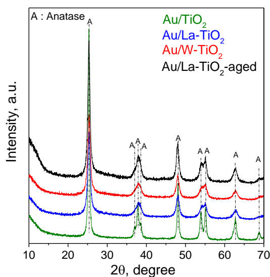
Figure 5.1 XRD patterns of Au/TiO 2 , Au/La-TiO 2 , Au/W-TiO 2 and Au/La-TiO 2 -aged catalysts.
