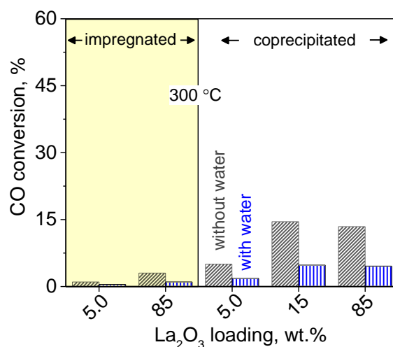
Figure 8.9 Effect of lanthana loading on the carbon monoxide oxidation activity of the gold catalysts in the presence and absence of 5 vol% water at 300 °C and W/F = 7.5*10 -5 g s cm -3 .
