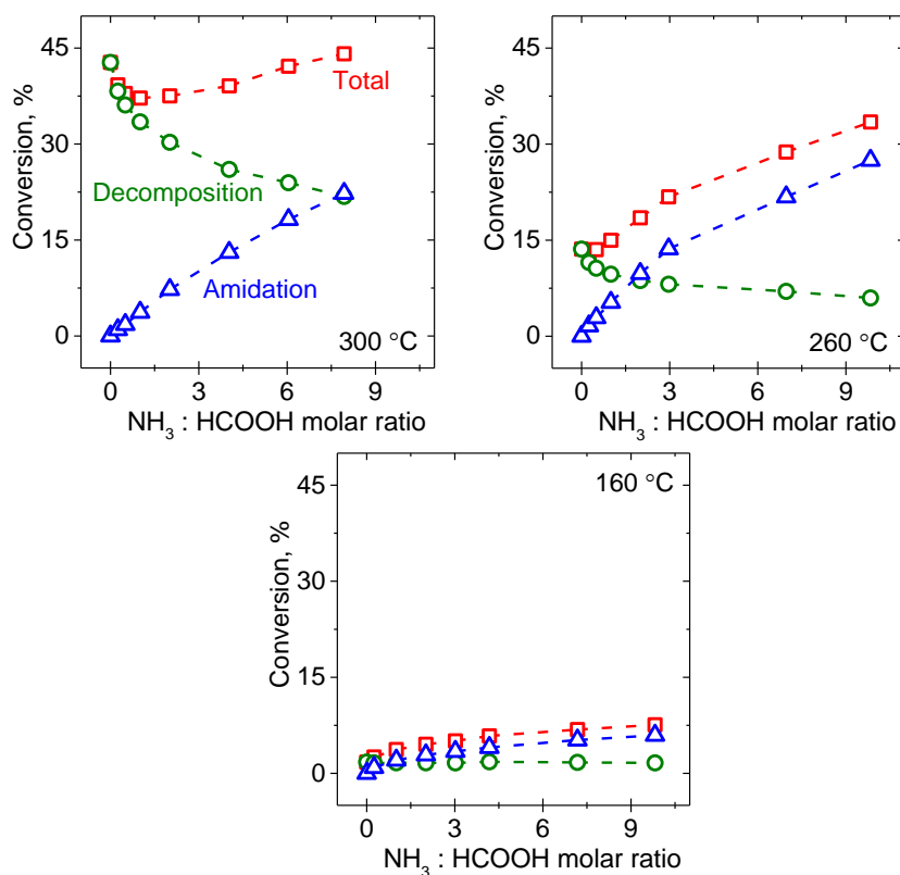
Figure 4.9 Trends in formic acid conversion over bare titania as a function of ammonia gas dosed in the feed stream for temperatures between 160 °C and 300 °C. ‘Decomposition’: formic acid conversion only to carbon dioxide and carbon monoxide. ‘Amidation’: formic acid conversion to methanamide and hydrogen cyanide. ‘Total’: sum of ‘Decomposition’ and ‘Amidation’.
