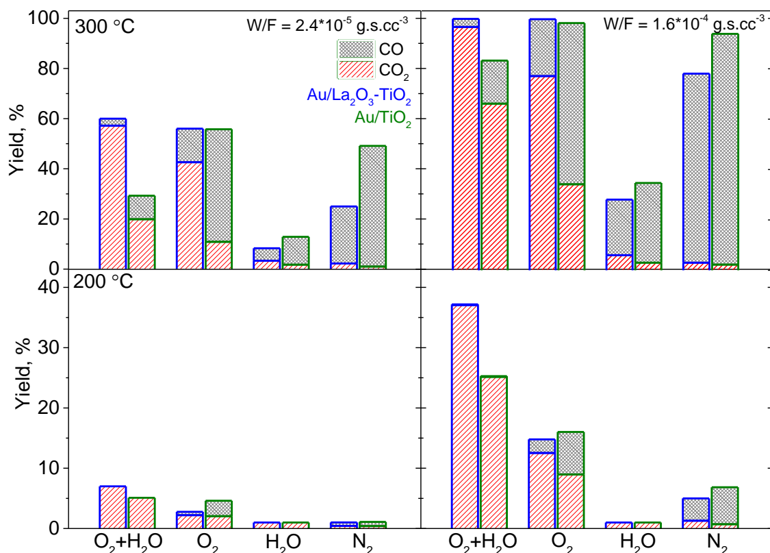
Figure 6.2 Comparison of carbon dioxide and carbon monoxide yield obtained from decomposition of 750 ppm formic acid over \text{Au/La-TiO}_2 and \text{Au/TiO}_2 using different feed compositions at 200 °C and 300 °C and W/F = 2.4 \times 10^{-5} \text{ g.s.cm}^{-3} (left column) and 1.6 \times 10^{-4} \text{ g.s.cm}^{-3} (right column).
