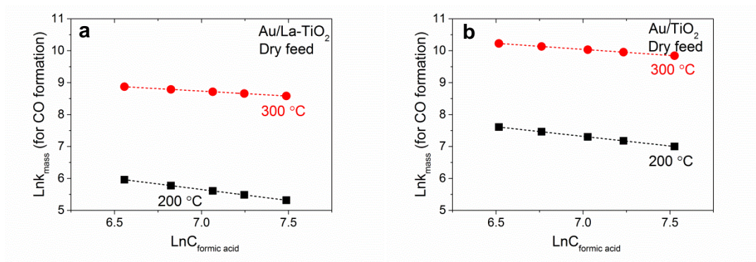
Figure 6.18 Plots used to calculate the apparent reaction orders at 200 °C and 300 °C for CO formation from formic acid decomposition in dry feed by varying formic acid concentration in the range 700-2, 200 ppm and (a) on Au/La-TiO 2 and (b) Au/TiO 2 .
