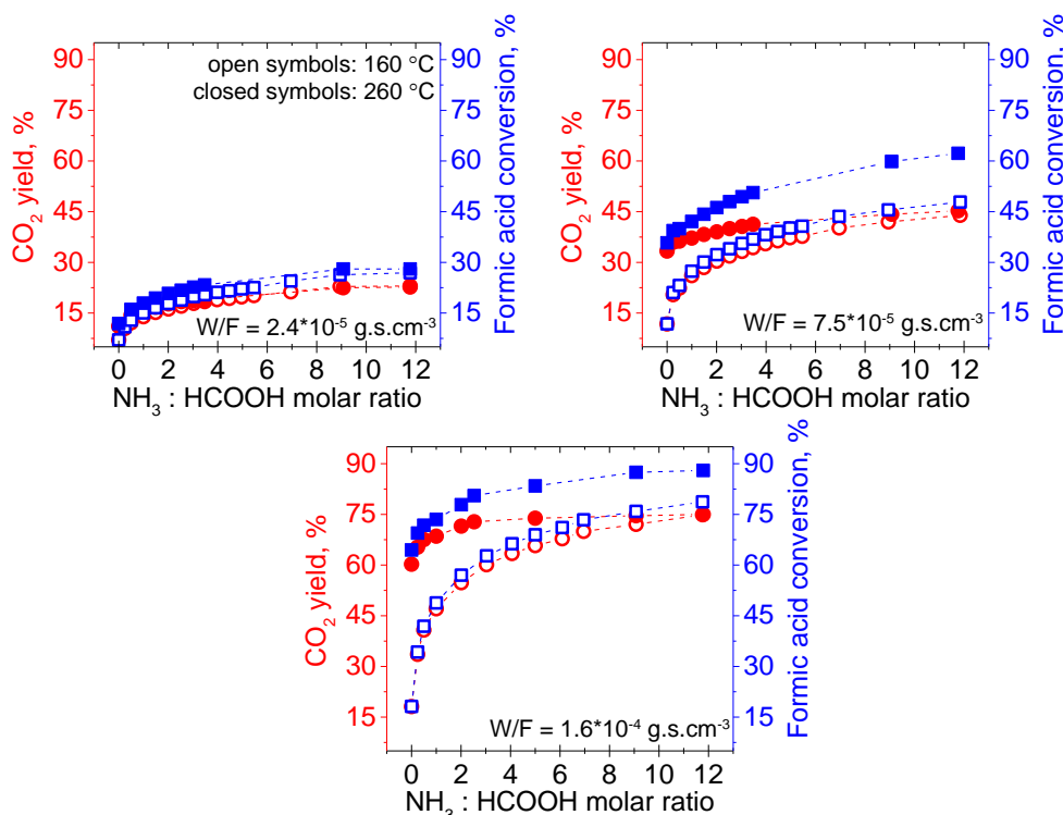
Figure 4.6 Formic acid conversion and carbon dioxide yield over 0.5 wt% Au/TiO 2 with varying ammonia to formic acid molar ratio at different temperatures: 160 °C (open symbol) and 260 °C (closed symbol) and different contact times.
