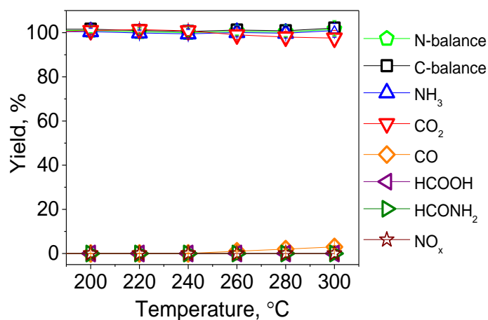
Figure. 3.4 Product yields for carbon dioxide, carbon monoxide, ammonia, formic acid, methanamide and nitrogen oxide (NO+NO 2 ) yields obtained upon the complete decomposition of 40% AmFo over 0.5 wt% Au/TiO 2 . (0.5 g·L -1 washcoat loading on the monolith, GHSV = 19,490 h -1 ; feed gas: 5 vol% water, 10 vol% oxygen, 85 vol% N 2 and 0.05 mL·min -1 liquid spray of 40 wt% AmFo).
