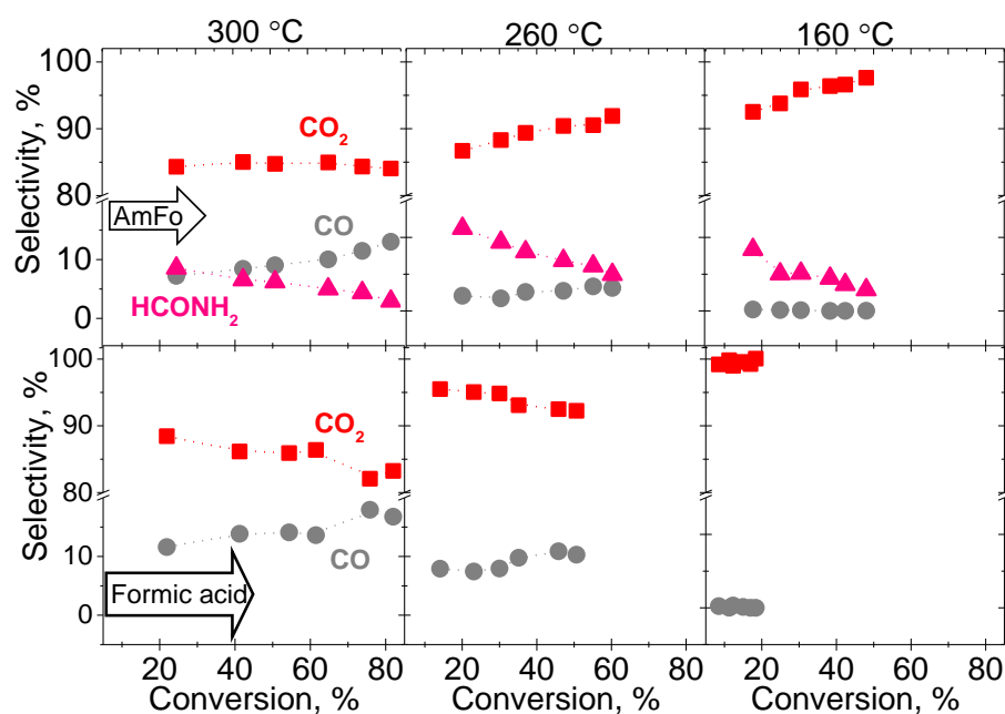
Figure 4.3 Selectivity versus conversion in the range 160 °C ≤ T ≤ 300 °C upon decomposition of AmFo (top) and formic acid (bottom) over 0.5 wt% Au/TiO 2 .
