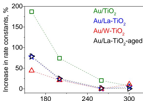
Figure 5.7 Effect of 1 molar equivalent of ammonia on formic acid decomposition rate constants over Au/TiO 2 , Au/W-TiO 2 , Au/La-TiO 2 and Au/La-TiO 2 -aged at W/F = 2.4 * 10 -5 g s cm -3 .
