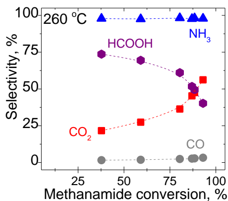
Figure 4.5 Selectivity versus conversion plot at 260 °C upon decomposition of 30% methanamide over 0.5 wt% Au/TiO 2 showing the formation of ammonia and formic acid as primary products upon methanamide hydrolysis followed by formic acid decomposition to carbon monoxide and carbon dioxide with increasing methanamide conversion.
