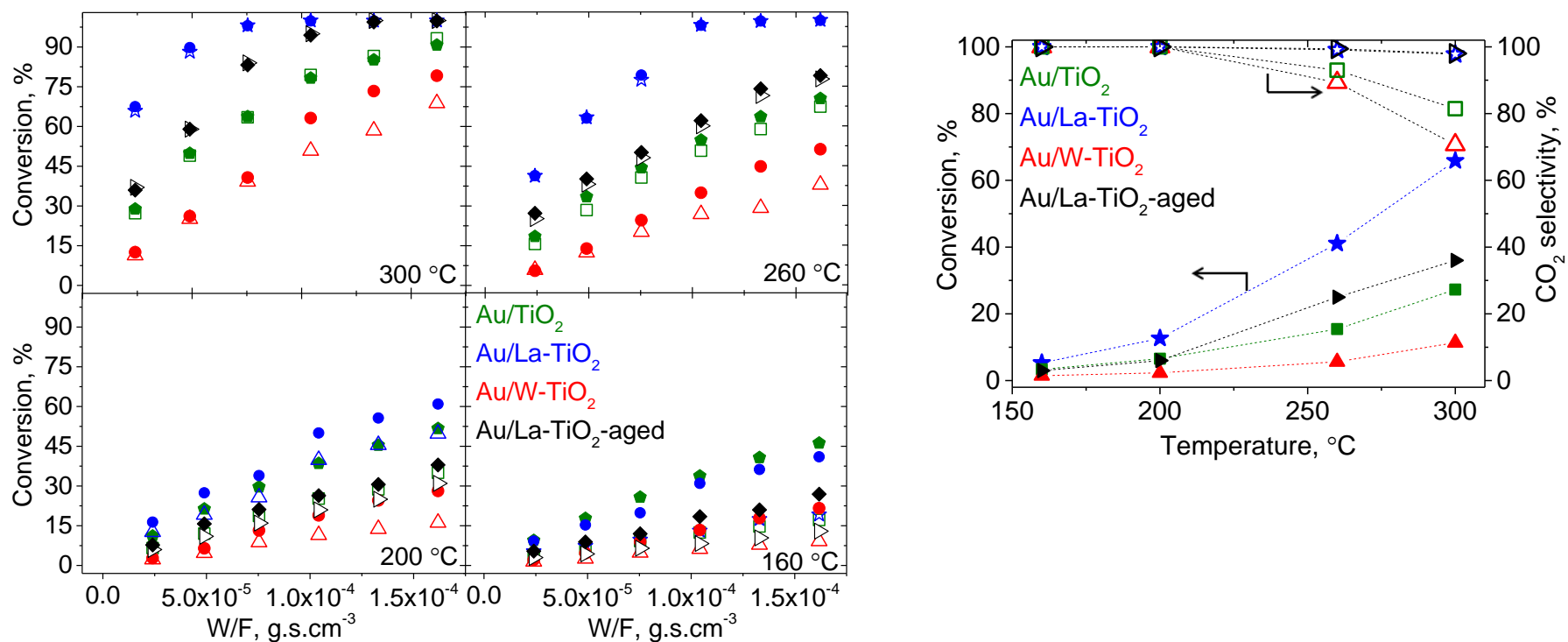
Figure 5.4 Formic acid conversion as a function of contact time, expressed as W/F (g s cm -3 ), obtained using AmFo (closed symbols) and formic acid (open symbols) at different temperatures (left) and temperature dependence of formic acid conversion (closed symbols) and carbon dioxide selectivity (open symbols) at W/F = 2.4*10 -5 g s cm -3 (right) over Au/TiO 2 , Au/W-TiO 2 , Au/La-TiO 2 and Au/La-TiO 2 -aged catalysts.
