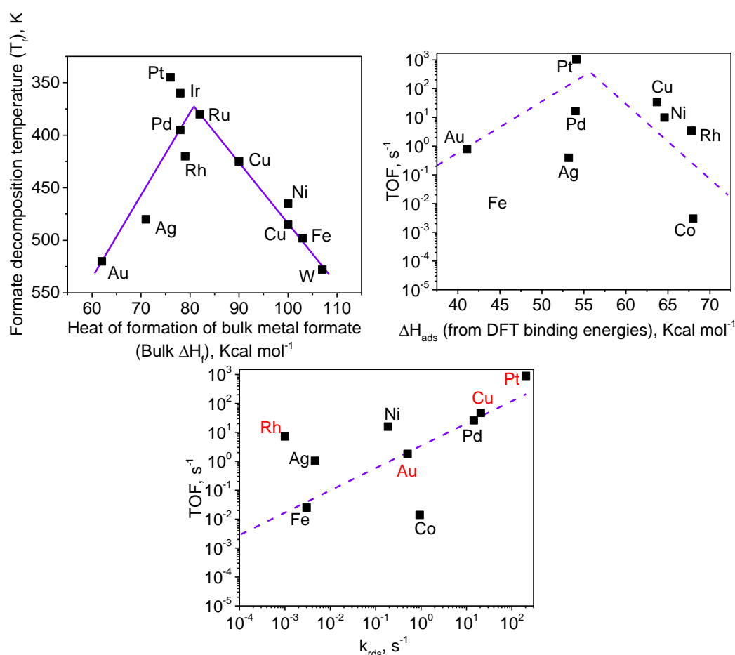
Figure 1.2 The original Sachtler–Fahrenfort volcano curve (top left), the plot of steady-state specific catalytic activity (TOF) for formic acid decomposition versus \Delta H_{ads} for surface formate from DFT calculations of formate binding energies on metal (111) surfaces (top right), and the plot of steady-state specific catalytic activity (TOF) for formic acid decomposition versus kinetics for surface formate decomposition ( k_{rds} ) bottom). Metals in black form monodentate surface formates and metals in red form bidentate/bridged surface formate. Adapted from Reference [40] , Copyright (2016), with permission from Elsevier.
