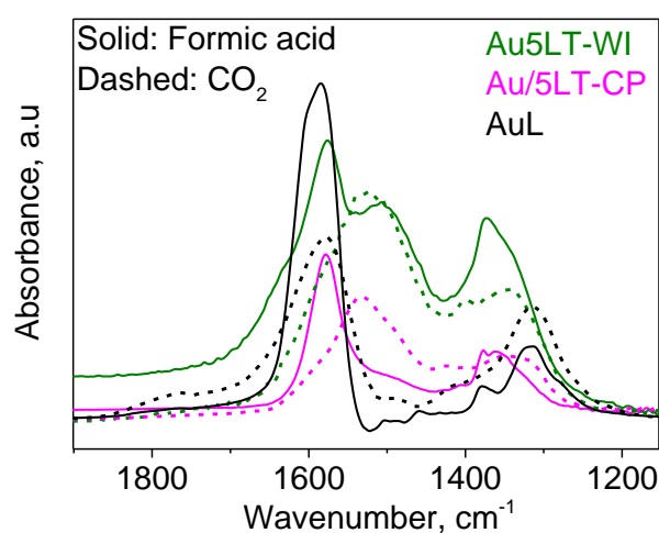
Figure 8.7 Comparison of in situ DRIFTS spectra of formic acid and carbon dioxide adsorption on selected catalysts.
