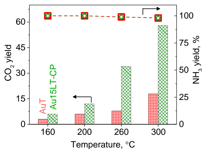
Figure 8.13 Ammonium formate decomposition on AuT and Au15LT-CP.
