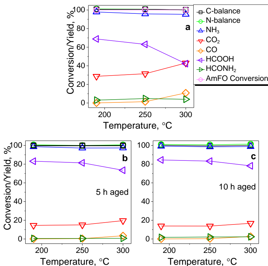
Figure 3.5 Product yields and AmFo conversion during AmFo decomposition over (a) fresh (b) 5 h aged, and (c) 10 h aged 0.5 wt% Au/TiO 2 catalysts (0.5 g·L -1 washcoat loading, GHSV = 19,490 h -1 ; feed gas: 5 vol% water, 10 vol% oxygen, 85 vol% N 2 and 0.05 mL·min -1 liquid spray of 40 wt% AmFo), showing nearly 100% ammonia yields between 200 °C and 300 °C.
