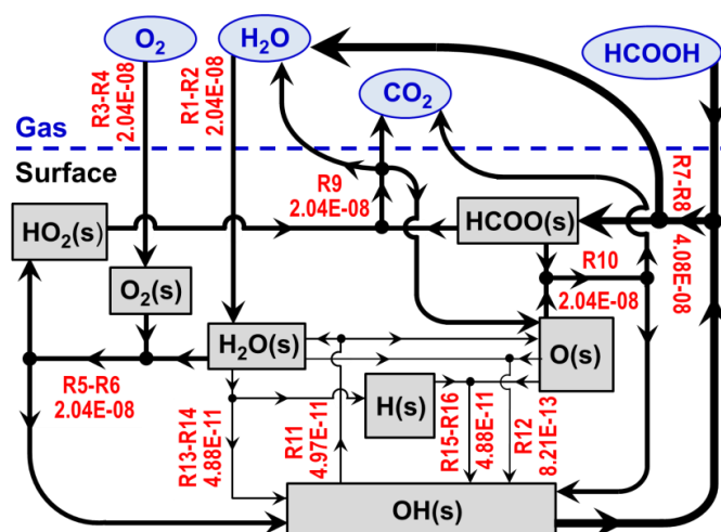
Figure 7.3 Reaction flux diagram for case I (Table 7.1) at 300 °C. Thicker lines (not to scale) denote dominant reactions.
