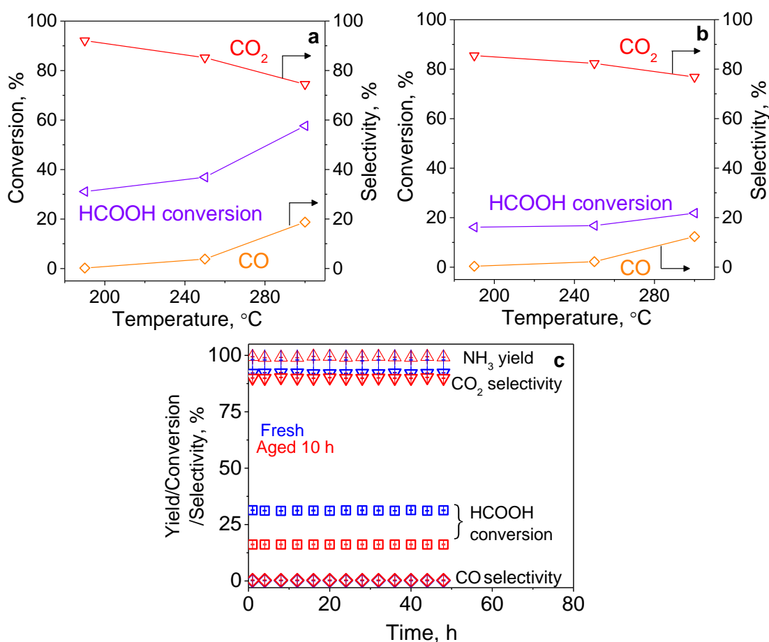
Figure 3.6 Relationship between selectivity and conversion with temperature for fresh (a) and 10 h aged (b) 0.5% Au/TiO 2 catalysts and (c) Time on stream plot portraying long term stability of fresh (blue) and 10 h hydrothermally aged (red) catalysts at 190 °C (0.5 g·L -1 washcoat loading on the monolith, GHSV = 19,490 h -1 ; feed gas: 5 vol% water, 10 vol% oxygen, 85 vol% N 2 and 0.05 mL·min -1 liquid spray of 40 wt% AmFo).
