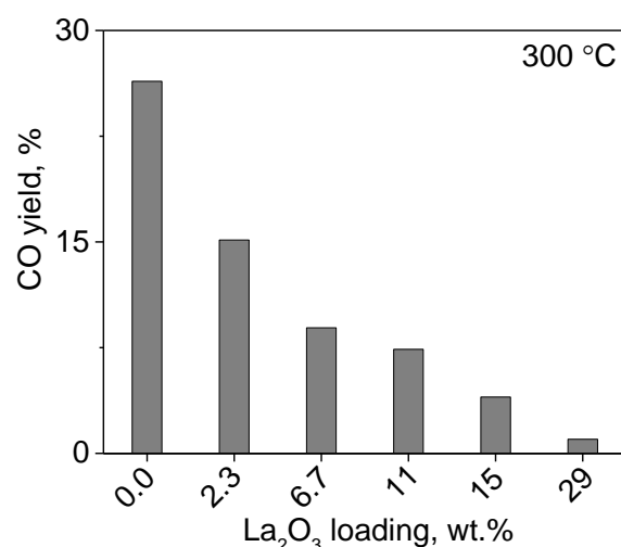
Figure 8.10 Effect of lanthana loading on the performance of supports prepared by coprecipitation for formic acid decomposition at 300 °C and W/F = 2.4 \times 10^{-5} \text{ g s cm}^{-3} .
