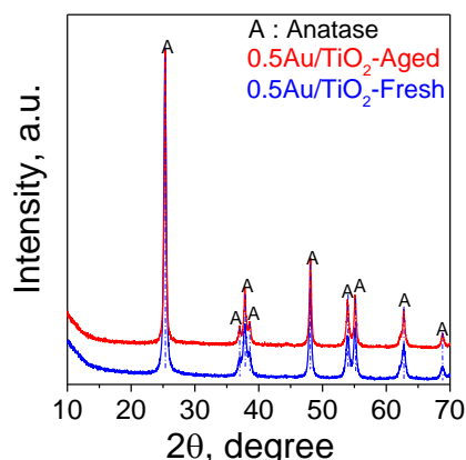
Figure 3.1 XRD patterns of fresh and 10 h hydrothermally aged 0.5 wt% Au/TiO 2 catalysts showing the absence of any major peaks associated with the rutile phase. The TiO 2 crystallite sizes were determined to be 25 nm and 32 nm in the fresh and 10 h hydrothermally aged samples, respectively.
