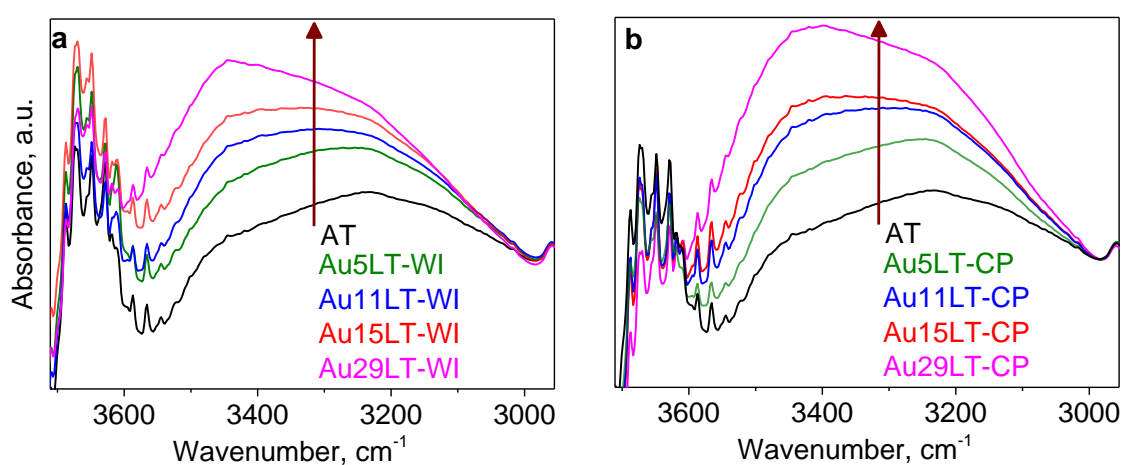
Figure 8.2 Absorbance in the hydroxyl region of (a) wet-impregnated and (b) coprecipitated catalysts.
