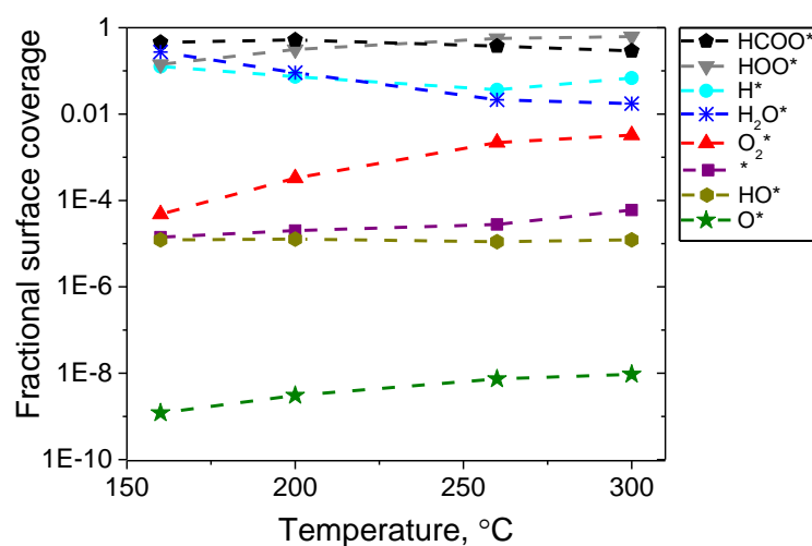
Figure 7.2 Predicted surface coverages as a function of temperature for Case I, Table 7.1.
