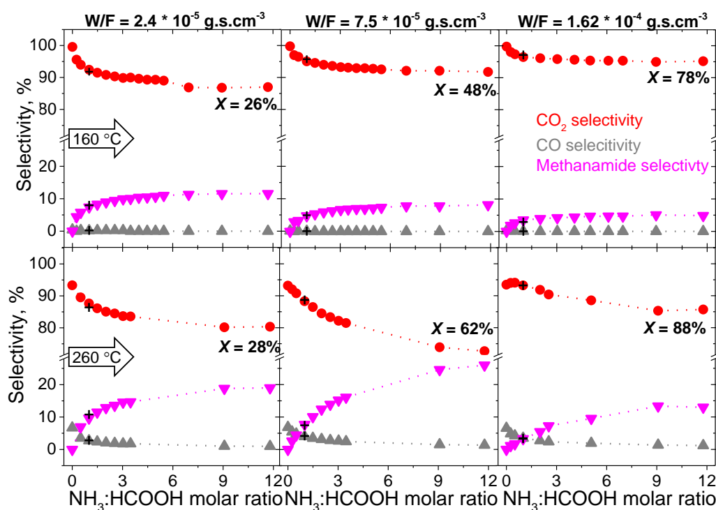
Figure 4.7 Carbon dioxide, carbon monoxide and methanamide selectivities obtained over 0.5 wt% Au/TiO 2 with varying ammonia to formic acid molar ratio at different temperatures: 160 °C (top row) and 260 °C (bottom row), and different contact times, the (+) symbols represent the corresponding selectivities obtained during AmFo decomposition.
