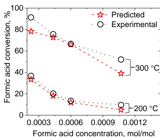
Figure 7.6 Simulated and measured trends in formic acid conversion as a function of formic acid concentration (Case II, Table 7.1) at 200 °C and 300 °C.
