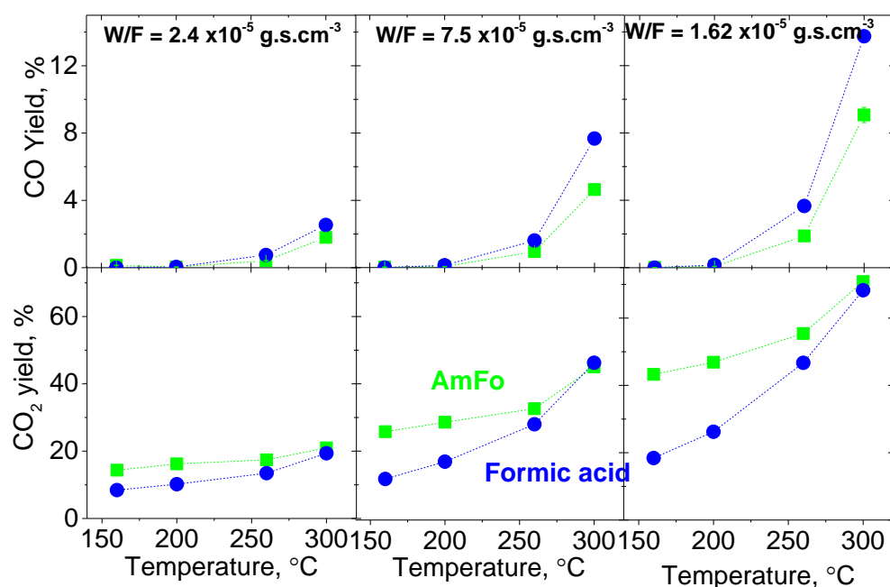
Figure 4.2 Evolution of carbon monoxide yields (top row) and carbon dioxide yields (bottom row) with temperature for different W/F upon decomposition of AmFo (green) and formic acid (blue) over 0.5 wt% Au/TiO 2 .
