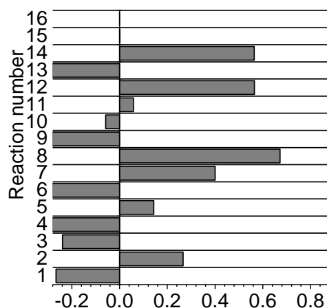
Figure 7.5 Sensitivity analysis for H^* in a surface perfectly stirred reactor (SPSR) for oxygen concentration of 0.01 mol/mol at 300 °C. Reaction numbering follows Table 7.2.
