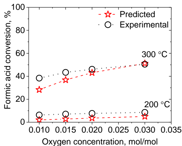
Figure 7.8 Simulated and measured trends in formic acid conversion as a function of oxygen concentration (Case III, Table 7.1) at 200 °C and 300 °C.
