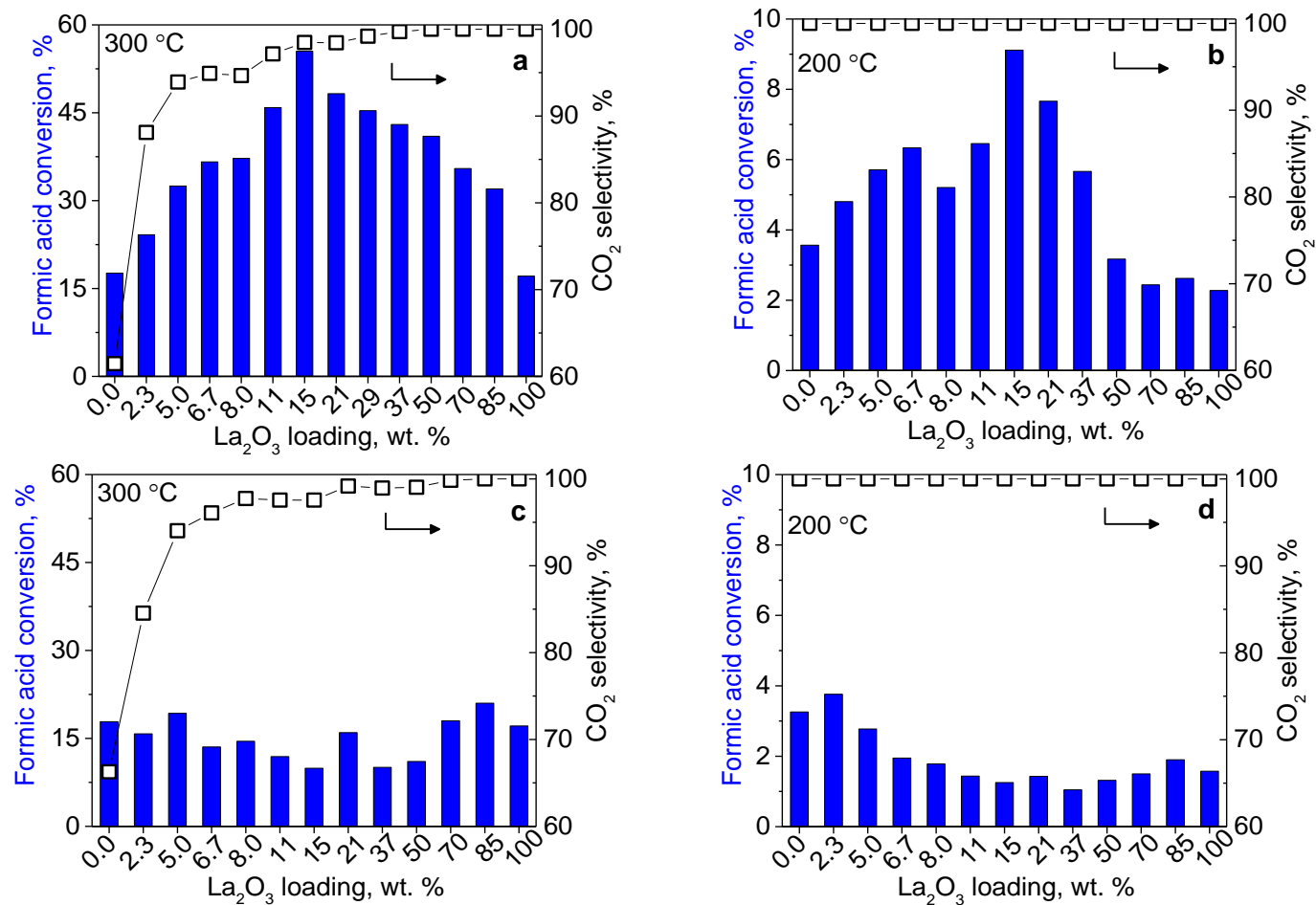
Figure 8.8 Effect of lanthana loading on the catalytic activity of gold catalysts prepared by (a,b) coprecipitation, and (c,d) wet-impregnation for formic acid decomposition at 200 °C and 300 °C and W/F = 2.4 \cdot 10^{-5} \text{ g s cm}^{-3}
