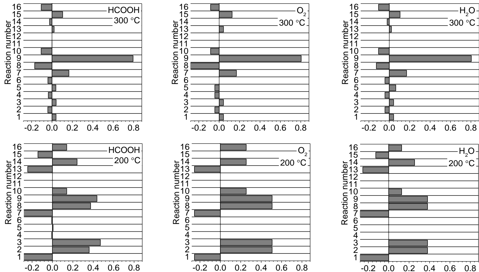
Figure 7.4 Sensitivity analysis for conversion of formic acid, oxygen and water, in a surface perfectly stirred reactor (SPSR) for case I in Table 7.1 at 300 °C and 200 °C. Reaction numbering follows Table 7.2.
