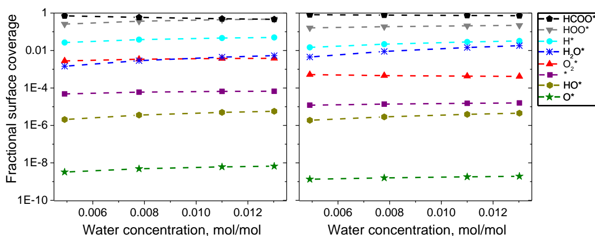
Figure 7.11 Predicted surface coverages as a function of water concentration (Case III, Table 7.1) at 300 °C (left) and 200 °C (right).
