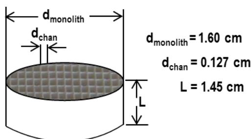
Scheme 7.1 Sketch of a model monolith and its dimensions.
