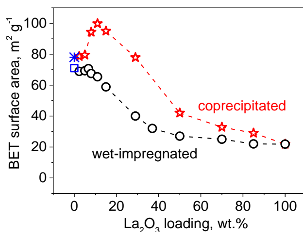
Figure 8.4 BET surface area (m 2 g -1 ) as a function of lanthana loading in the gold catalysts prepared via coprecipitation and wet impregnation. The blue square and star represent AuT and AuT-MA, respectively.
