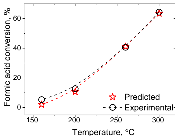
Figure 7.1 Comparisons of predicted and measured formic acid conversions as a function of temperature for Case I, Table 7.1.
