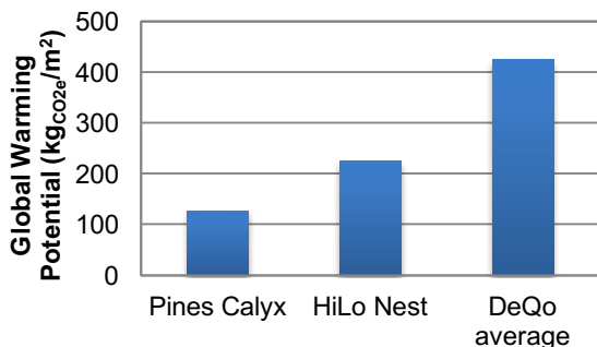
Fig. 5: Comparison of the embodied carbon.
