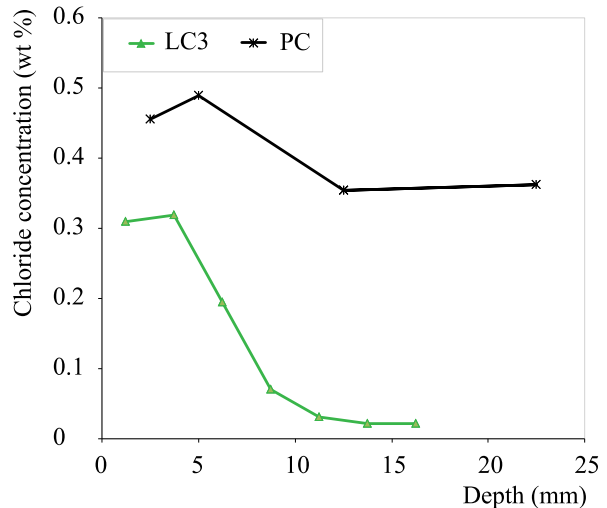
Fig. 3: Chloride profiles after 2 years ponding in 0.5M NaCl.
