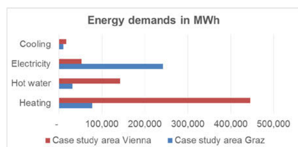
Fig. 2: Energy demands in case study areas.
