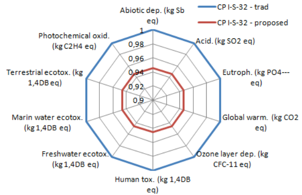
Fig. 3: Impacts of 1 ton of cement CP I-S-32, using avoided burden vs. proposed approach.
