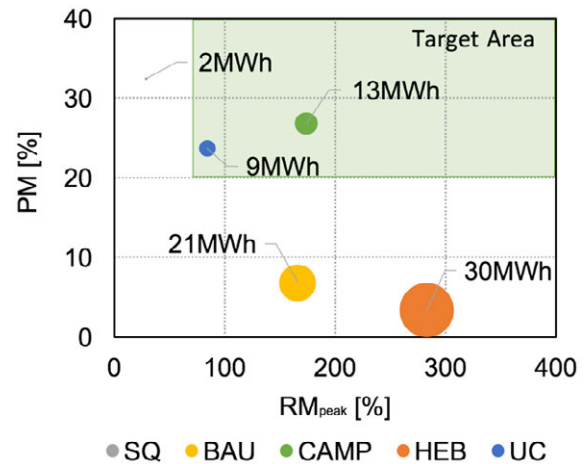
Fig. 3 The resilience of energy systems. In this figure, the size of the bubble represents the total electricity storage per scenario.
