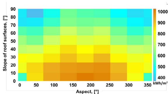
Fig. 5: Yearly mean solar irradiation [ \text{kWh/m}^2 year] as a function of the slope [ 0-90^\circ ] (y-axis) and aspect [ 0-360^\circ ] (x-axis) of the roof surfaces for the city of Geneva.
