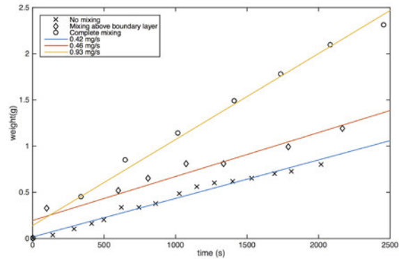
Fig. 1: Adsorption of liquid desiccant as a function of different airflows above contact surface.
