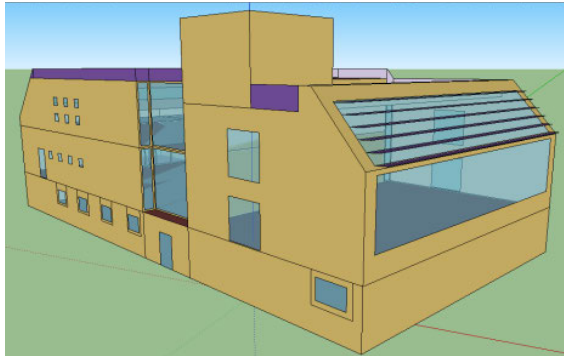
Fig. 3: Building energy model in EnergyPlus.
