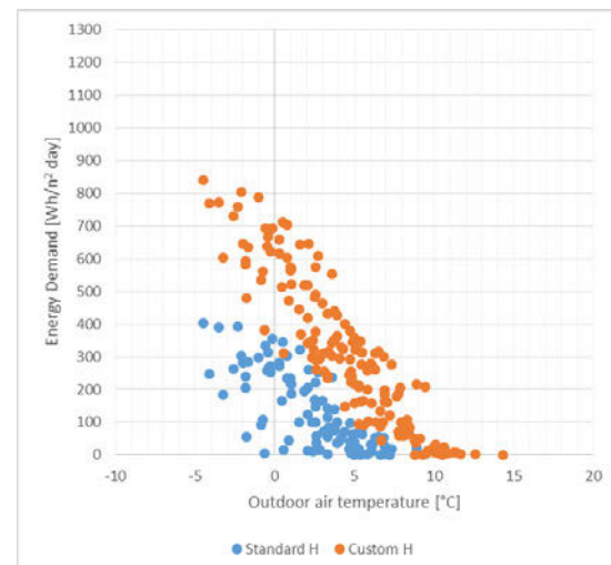
Fig. 7: Heating demand with standard occupancy profile and custom behavioural pattern.
