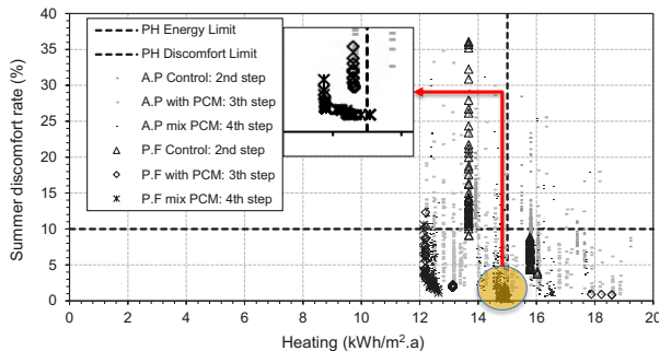
Fig. 5: Optimized results: 4 th step.
