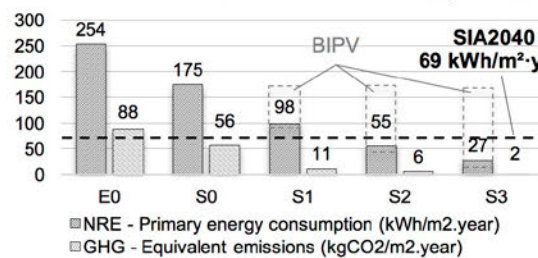
Fig. 4 Net energy consumption and emissions.
