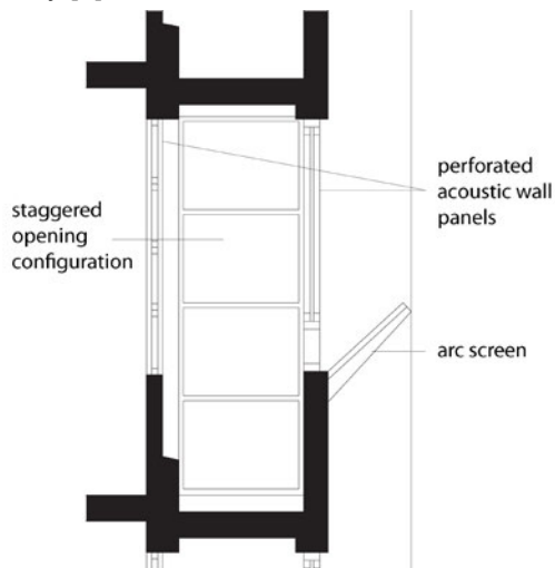
Fig. 7: Section Acoustic Balcony © Hong Kong Housing Authority, graphics modified by © Ferdinand Oswald, 2013.
