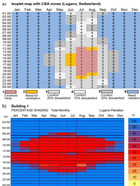
Fig. 4: a) Isoleth map with CBA zones (1-6) represented. The black line identified the period of time where shadow is necessary to prevent overheating; b) Shading graphic example calculated for Building 1.
