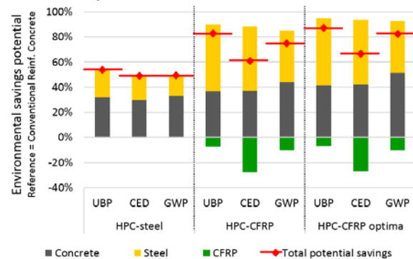
Fig. 2: Environmental impact assessment of 1 linear meter HPC-CFRP beam structure. Reference is conventional reinforced concrete. HPC and reference are modelled using OPC while HPC optima is modelled using cement with 40% clinker. Beam design is based on Table 2 .
