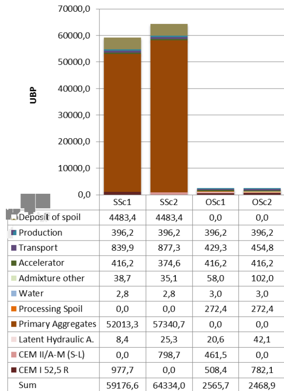
Fig. 2: Comparison of mineral resources (EP).
