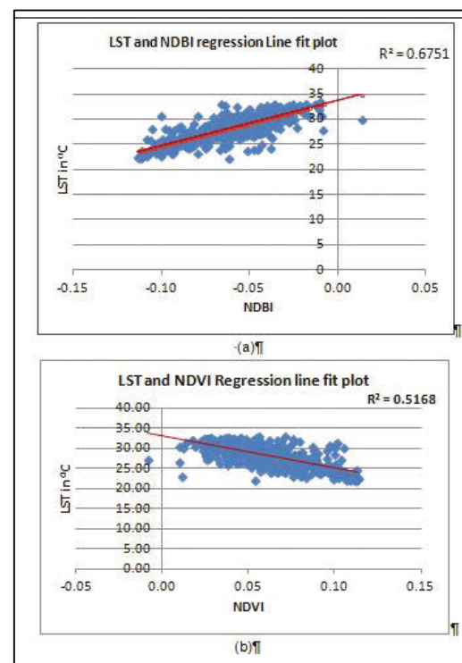
Fig. 7: Above figures show a grid wise regression line plot between (a) LST and NDBI (b) LST and NDVI for each grid of 'S' ward.
