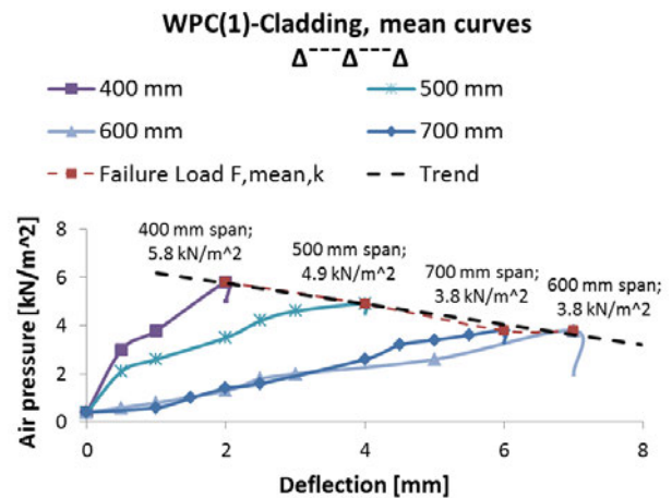
Fig. 6: Load curves of Product 1.
