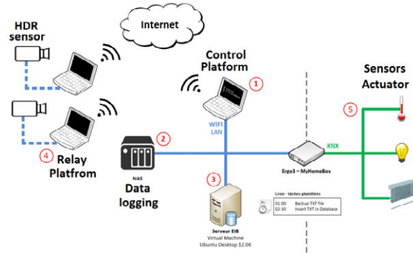
Fig. 2: Communication platform layout.
