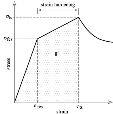
Fig. 3: Strain hardening with multiple cracking in UHP-FRCC.
