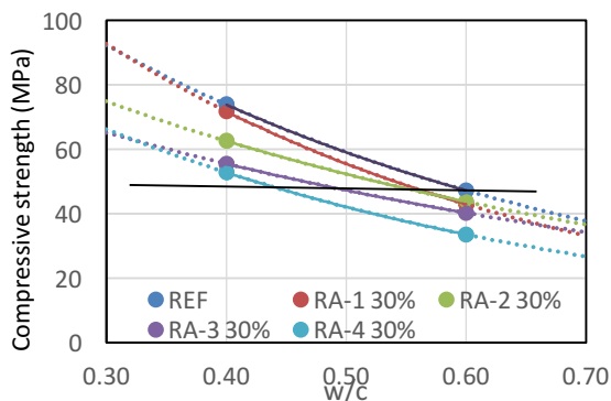
Fig. 6: Efficiency of 30% aggregate replacement - Strength.
