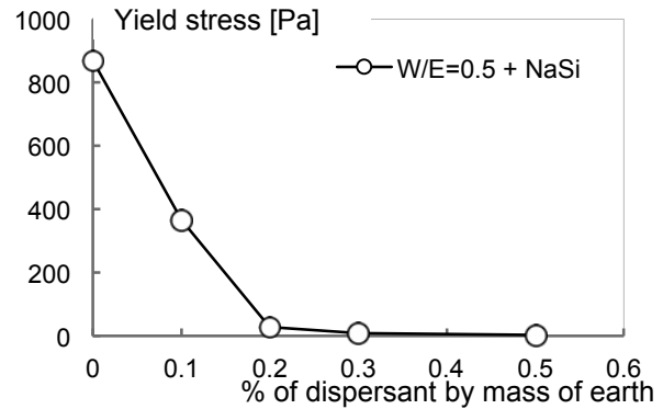
Fig. 1: Effect of NaSil on the yield stress of earth paste.
