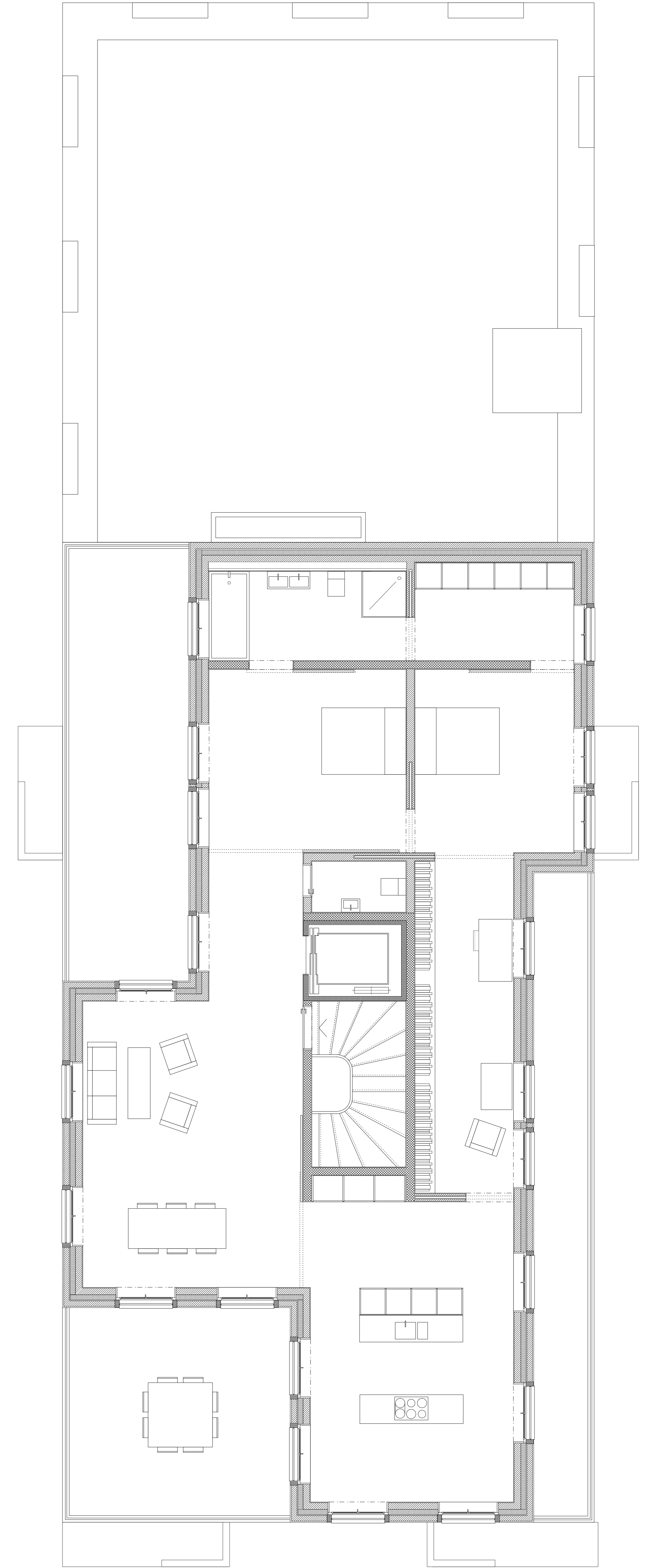
Attikageschoss 1:50
