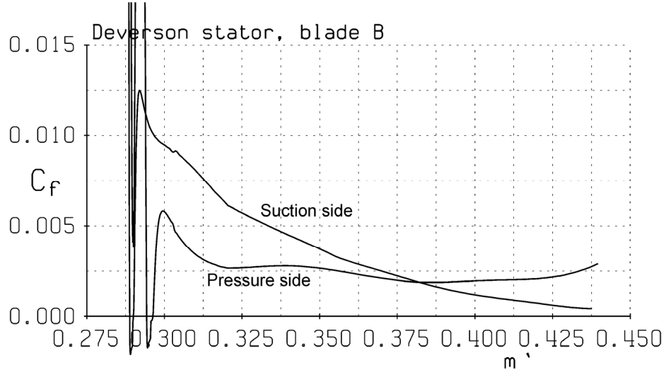
Figure 4.2-2: Mises analysis of blade B
