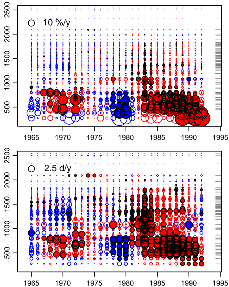
Figure 2.2: Time-height section of decadal Swiss snow day trends. Upper panel: relative 15-year running window trends (units:%/yr), lower panel: absolute 15-year running window trends (units: days/yr). Blue (red) circles show positive (negative) trends. Significant trends according to a two sided t-test on the 10% level are filled and have a black border. The height distribution of the snow stations is indicated by dashes on the right side. A scale for the circles is shown in both panels.
