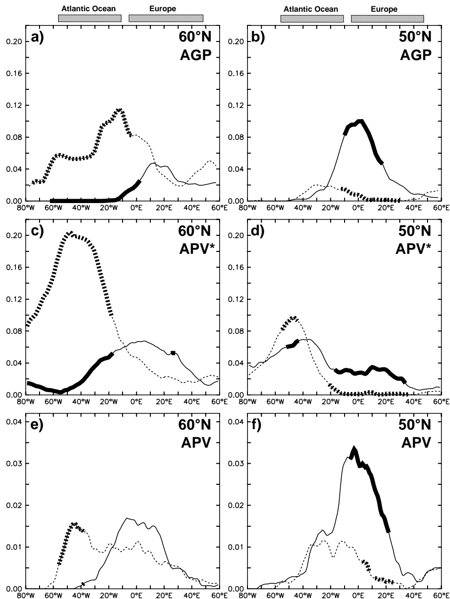
Figure 4.4: Blocking frequency sections at 60°N (left panels) and 50°N (right panels) for the NAO+ tercile (solid lines) and the NAO- tercile (dashed). Results are shown for AGP (a, b), APV* (c, d) and for APV (e, f). Longitudes showing significantly increased or decreased blocking frequencies are indicated in bold. The frequencies shown are slightly boxcar smoothed (three point smoother). Note that the ordinate runs from 0 to 0.2 for AGP and APV* but from 0 to 0.04 for APV.
