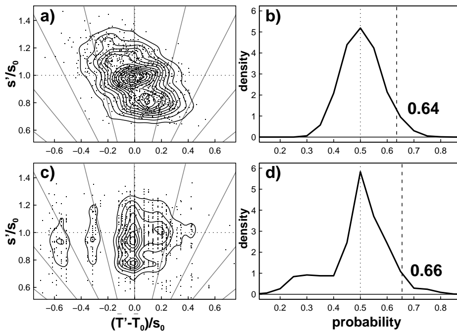
Figure 5.2: Bootstrapped uncertainty estimates for the DJF 61–90 northern Switzerland temperature normal definition. The MSC plots show estimates based on a) mean and standard deviation and c) median and IQR/1.349. For display purposes 1000 bootstrap samples are shown as dots. The density values are based on 5000 samples (contour lines, levels as in Figure 5.1). The corresponding PDFs of the PPA are shown in panel b) and d). The 95 th percentile confidence limit for the mean-standard deviation (median-IQR/1.349) estimator is 0.64 (0.66).
