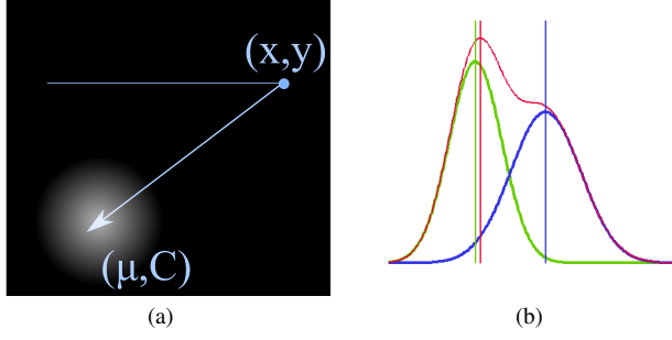
Fig. 1 (a) Illustration of a supporter voting for a target position (arrow) with a probability distribution (image intensities) defined by mean \boldsymbol{\mu} and covariance \mathbf{C}_s . (b) Illustration of a 1D Gaussian Mixture Model (red) from two individual distributions (green and blue), with mean values indicated by vertical lines.
