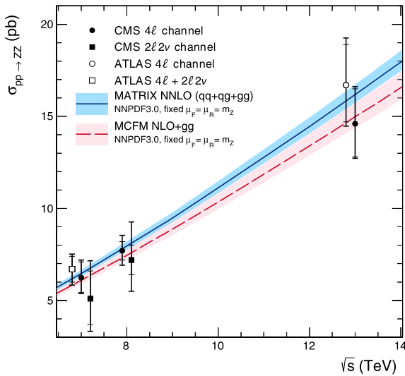
Fig. 5. The total ZZ cross section as a function of the proton–proton center-of-mass energy. Results from the CMS and ATLAS experiments are compared to predictions from MATRIX and MCFM with NNPFD3.0 PDF sets and fixed scales \mu_F = \mu_R = m_Z . Details of the calculations and uncertainties are given in the text. Measurements at the same center-of-mass energy are shifted slightly along the x-axis for clarity.
