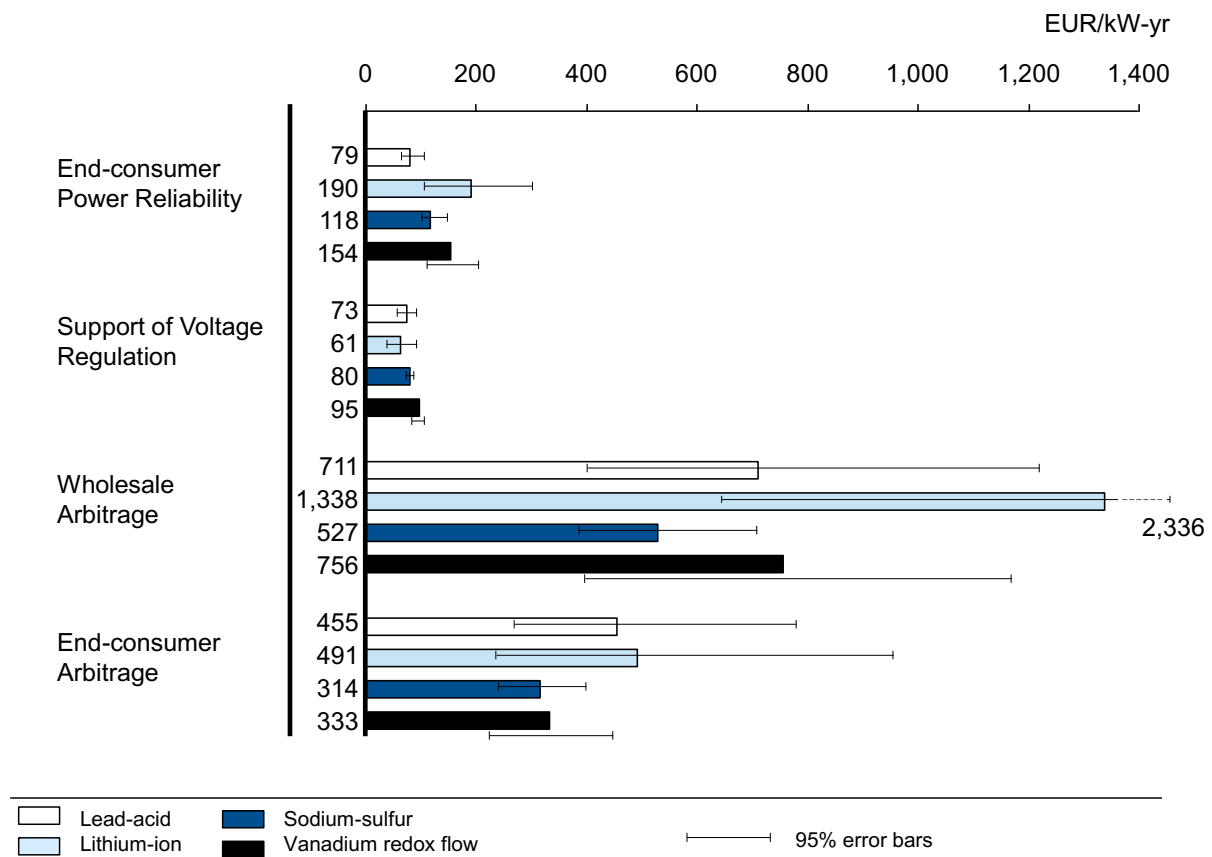
Figure D.1 – Levelized costs of electric capacity (LCOEC) of battery technologies across applications 38
