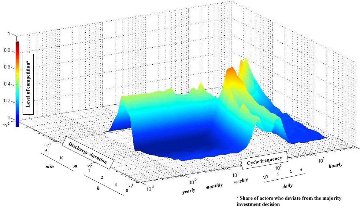
Figure E.1 – Degree of competition among battery technologies in the application landscape (3D)
