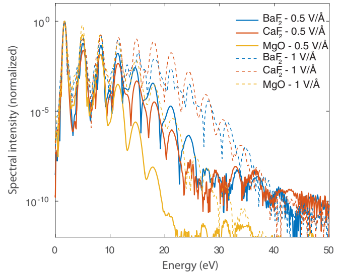
FIG. 5. HHG as a general feature of strong-field-driven solids. Simulated HHG spectra of different crystals being driven by different peak electric fields (shown in the legend). The crystal orientations are selected to have the maximum spectral response. In this case, they are all oriented such that the input laser polarization is parallel to \Gamma - L .
