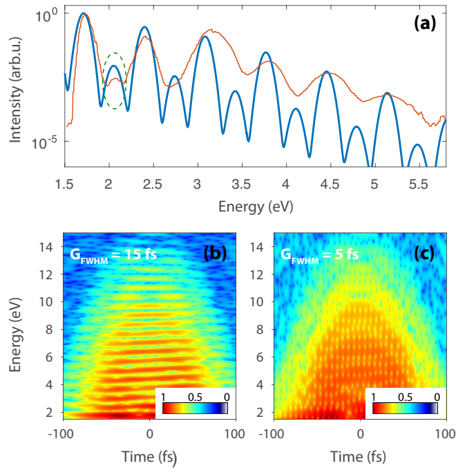
FIG. 4. Spectra and temporal characteristics of HHG from ZnO. (a) Simulated HHG spectrum of ZnO (solid dark blue line), plotted in the same spectral range as the experimental spectrum [14] (solid orange line). The oval dark green dashed line highlights the weak sixth-order harmonic that was also detected in experiment. (b) (Logarithmic scale) Time-frequency analysis of the generated temporal profile using a Gaussian with width G_{\text{FWHM}} = 15 fs. (c) (Logarithmic scale) Same time-frequency analysis with a Gaussian width G_{\text{FWHM}} = 5 fs.
