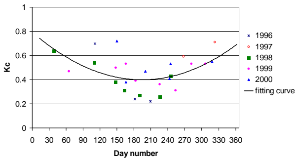
Figure 11: Spatially averaged K_c values of the catchment plotted against day number of the year.
