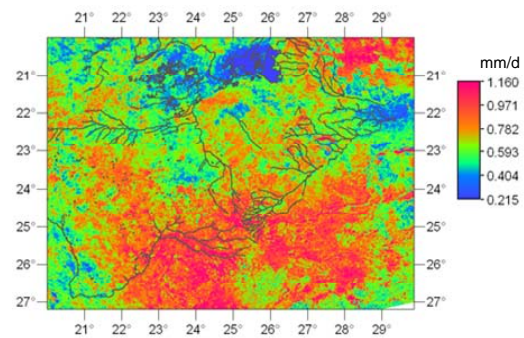
Figure 2: Actual ET_{24} map calculated from NOAA 14 AVHRR image on 09/07/1998.
