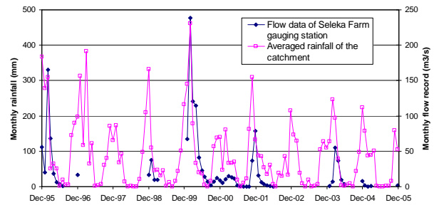
Figure 7: Flow data from Seleka Farm gauging station plotted against monthly rainfall in the catchment.
