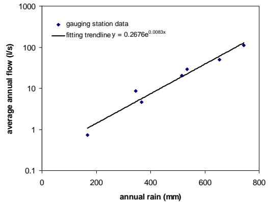
Figure 8: Annual flow from Seleka Farm gauging station plotted against annual accumulated rainfall.
