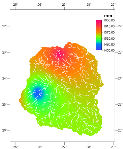
Figure 14: Annual potential ET of the catchment, averaged over the period from 1996 to 2005.
