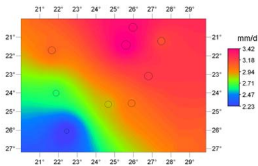
Figure 1: Potential ET calculated from meteorological station data with moving average interpolation on 09/07/1998.
