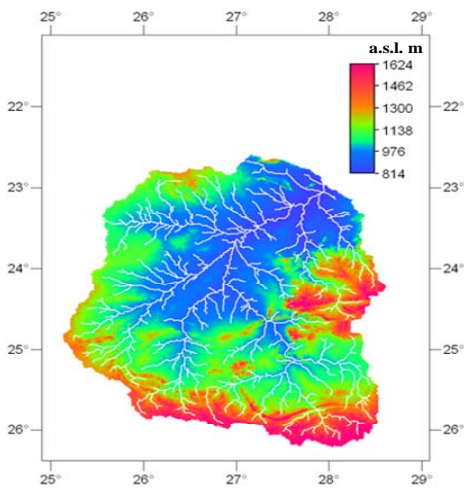
Figure 6: Catchment above Seleka Farm gauging station and drainage network.
