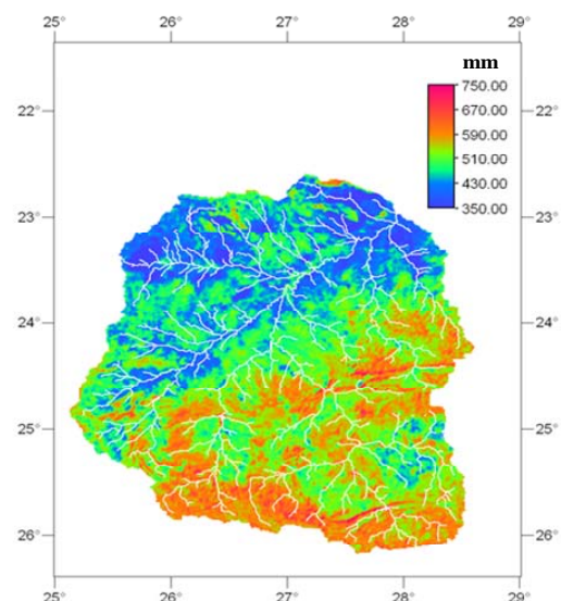
Figure 15: Annual ET map
