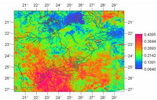
Figure 3: K_c map calculated from ET_{24} map and ET_0 map for 09/07/1998.
