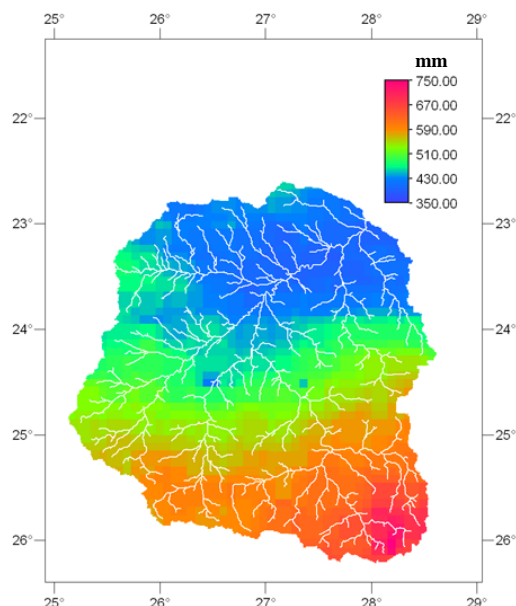
Figure 16: Annual precipitation of the catchment averaged over 10 years from 1996 to 2005.
