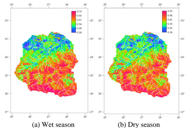
Figure 9: Five-year-average K_c map of the catchment in wet season and dry season.
