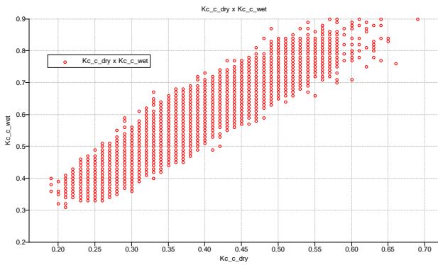
Figure 10: Cross correlation of the K_c maps in wet and dry seasons
