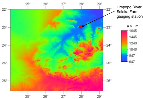
Figure 5: DEM map of Kanye region with location of the gauging station Seleka Farm on the Limpopo River.
