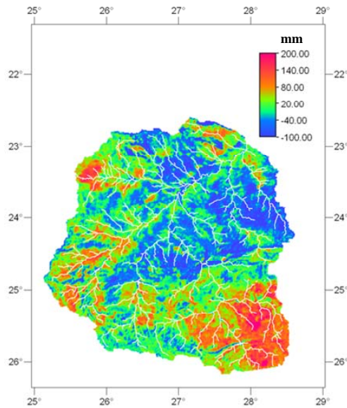
Figure 17: Averaged annual Precipitation-ET map
