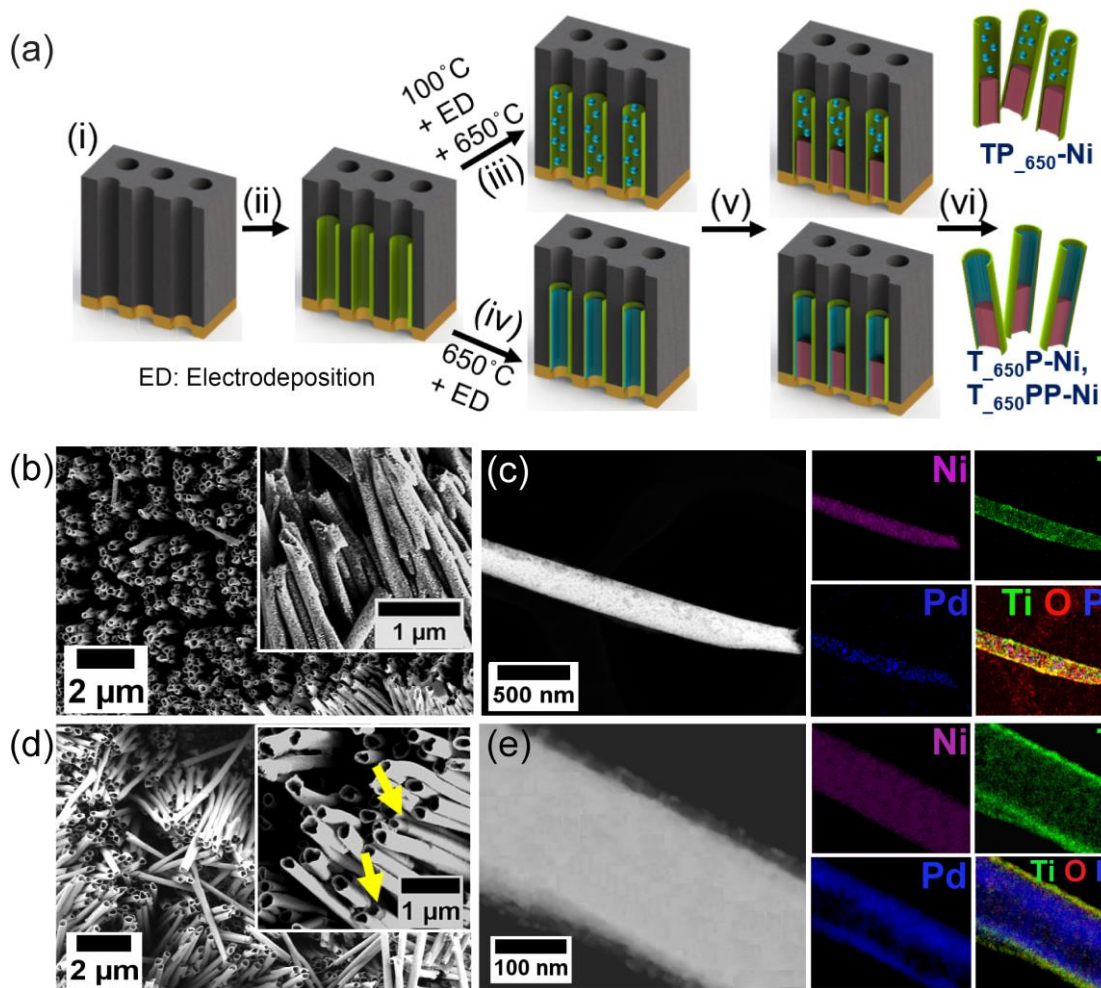
Figure 1. Fabrication overview of hybrid NTs: (a) (i) Au sputtered on one side of AAO templates, (ii) electrochemically induced sol-gel deposition of \text{TiO}_2 NTs, (iii) electrodeposition (ED) of Pd NPs inside \text{TiO}_2 NTs dried at 100\text{ }^\circ\text{C} , followed by annealing at 650\text{ }^\circ\text{C} , (iv) electrodeposition of Pd NTs inside \text{TiO}_2 NTs annealed at 650\text{ }^\circ\text{C} , (v) electrodeposition of Ni NWs, followed by (vi) etching of AAO templates. (b) SEM image showing an overview of freestanding \text{TP}_{650} NTs and the inset shows its magnified image with presence of NPs distributed on the \text{TiO}_2 surface. (c) HAADF STEM image of a single \text{TP}_{650}\text{-Ni} NT and its corresponding EDX Maps obtained for Ni, Ti, Pd and a superimposed image that clearly shows the presence of Pd as NPs inside a \text{TiO}_2 NT. (d) SEM image showing an overview of freestanding \text{T}_{650}\text{P} NTs and the inset shows its magnified image. (e) HAADF STEM image of a single \text{T}_{650}\text{P-Ni} NT and its corresponding EDX maps obtained for Ni, Ti, Pd where the superimposed image clearly shows a coaxial \text{TiO}_2\text{-Pd} NT structure.
