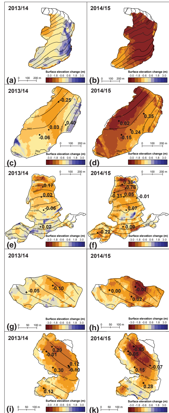
Figure 4. Spatial distribution of TLS-derived annual surface elevation changes \Delta h_{TLS} for (a, b) Glacier de Prapio, (c, d) Glacier du Sex Rouge, (e, f) St. Annafirn, (g, h) Schwarzbachfirn, and (i, k) Pizolgletscher in 2013/14 and 2014/15. The numbers indicate the differences (in m) between TLS-derived and in situ measured annual elevation changes at ablation stakes ( \Delta h_{TLS} minus \Delta h_{direct} ). White areas correspond to lidar shadow.
