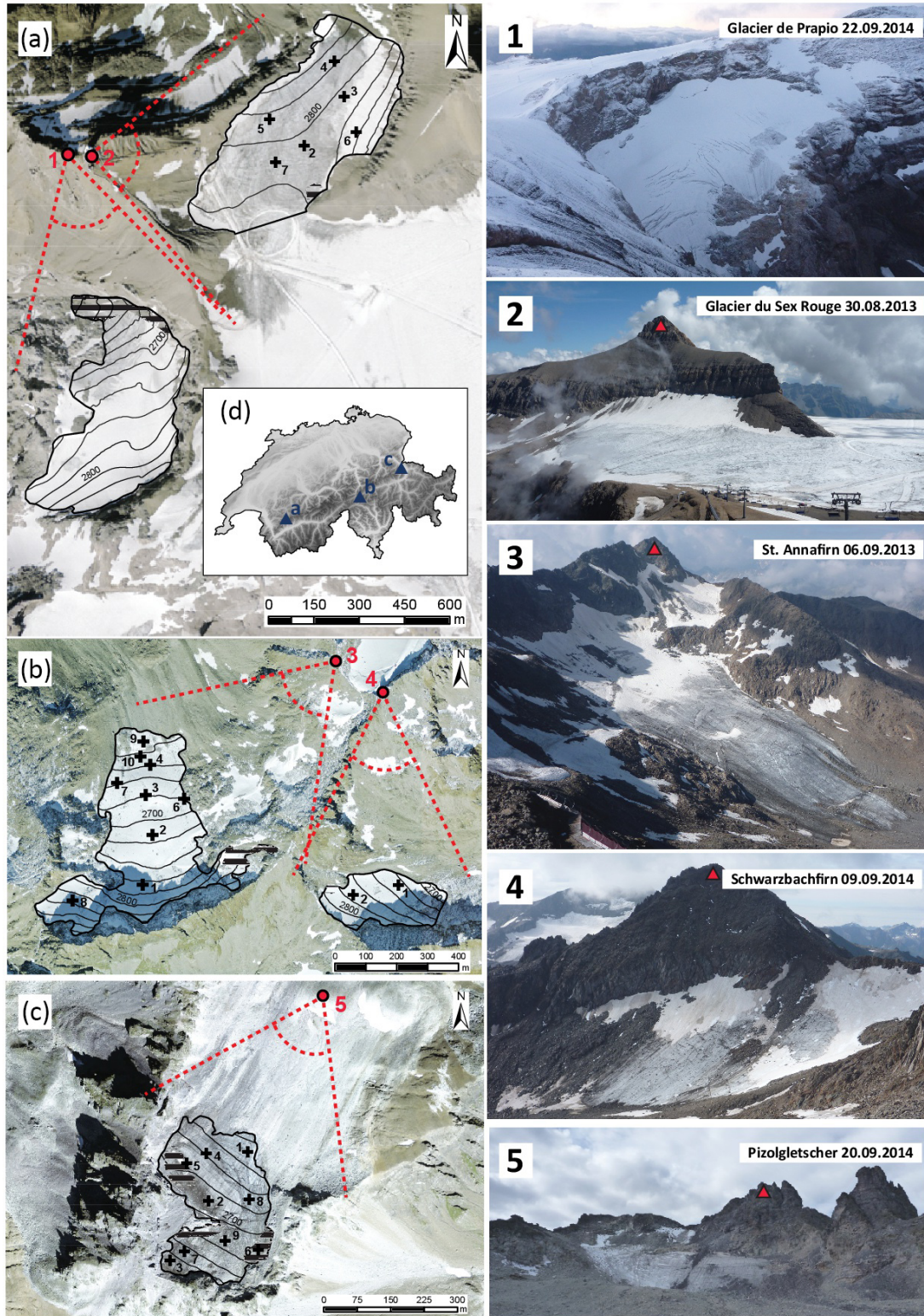
Figure 1. Overview of study sites. (a) Glacier de Prapio and Glacier du Sex Rouge, (b) St. Annafirn and Schwarzbachfirn, and (c) Pizolgletscher. The locations of the surveyed glaciers in the Swiss Alps is given in (d). Scan positions and horizontal view angles of the TLS surveys are shown by red dots and red dashed lines. Red numbers (on left side) correspond to individual photographs of the study glaciers (on right side) which were taken from the respective scan positions. Red triangles on the photographs refer to summits mentioned in the text. Black dashed areas indicate lidar shadow, and black crosses the locations of ablation stakes.
