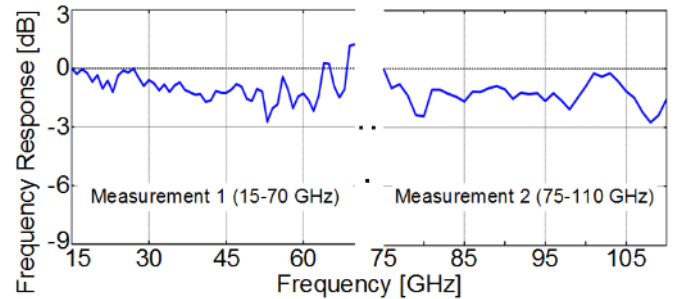
Fig. 12 High-speed RF-measurement Electro-optic frequency response of an all-plasmonic MZM. Two separate measurements were performed for the lower (15-70 GHz) and the higher frequency (75-110 GHz) range. Each measurement was normalized to its starting frequency at 15 GHz and 75 GHz, respectively. No bandwidth limitation can be observed beyond the measurement range of 110 GHz.
