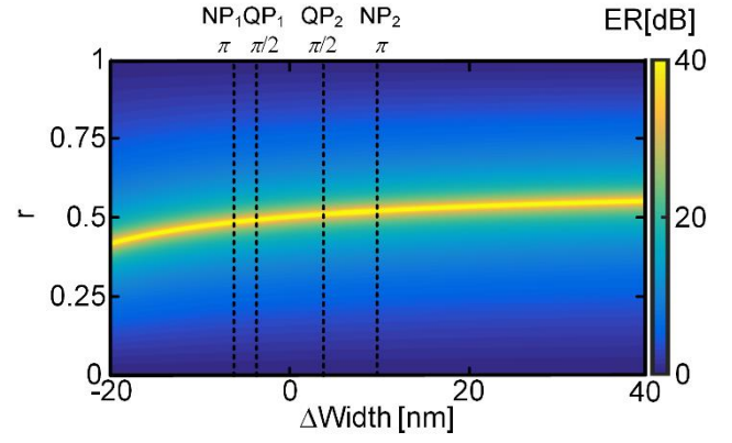
Fig. 9 Extinction Ratio as a function of the splitting ratio r and a slot asymmetry. The dashed lines indicate slot width differences resulting in a phase difference between the two Mach-Zehnder arms in the amount of \pi and \pi/2 . This phase differences correspond to operations in the null point (NP) and quadrature point (QP), respectively. The inherent reduction of the ER for unequal slot widths in these operation points is uncritical since the ER remains high in all cases. Only for large slot width differences the splitting ratio r has to be adapted to maintain high ERs.
