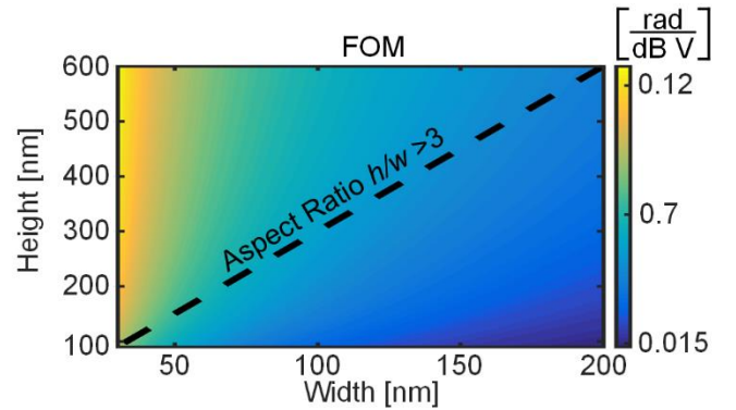
Fig. 7 Figure-of-Merit: The plot shows the achievable FOM as a function of the slot's height and width. The FOM shows how much phase shift can be accumulated per 1 dB propagation loss and 1 V applied voltage. The dashed line indicates an aspect ratio ( h/w ) of 3. This line marks the current fabrication limits. Aspect ratios above 3 – even though more promising – are difficult to fabricate.
