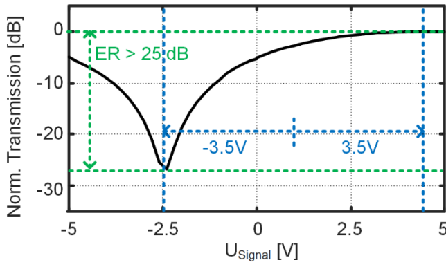
Fig. 10 MZM transfer function: Normalized transmission plotted as a function of the drive voltage ( U_{\text{signal}} ) for phase shifters of 6 \mu\text{m} length. The measurement reveals record low voltage-length product of 40 \text{ V}\mu\text{m} . The large Extinction ratio confirms that the small-footprint enables symmetric interferometers.
