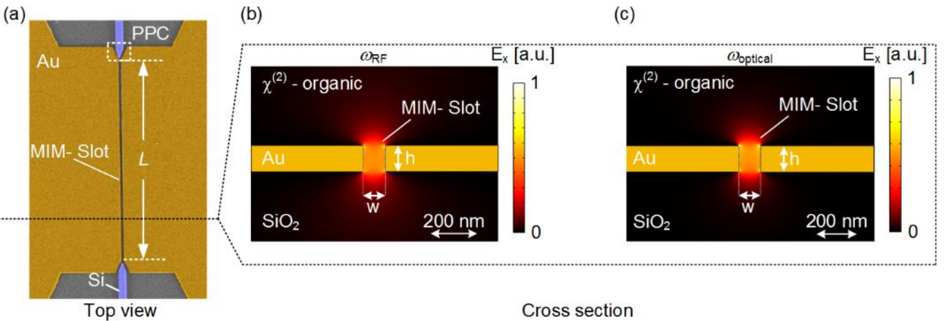
Fig. 5 Plasmonic phase modulator: (a) shows a colorized SEM image of the phase modulator. Au is indicated in yellow, silicon in blue and SiO 2 is given in gray. The two Au contact pads form the MIM slot waveguide, which is filled with the organic material. Light is coupled to and from the slot by Plasmonic-Photonic couplers (PPCs). The cross section with the RF and optical fields are shown in (b) and (c) for a slot with height ( h ) and slot width ( w ) of 150 nm and 100 nm, respectively. Both images show the simulated E_x component at optical and RF-frequency, respectively. Their perfect overlap suggests the strongest possible light-matter interaction.
