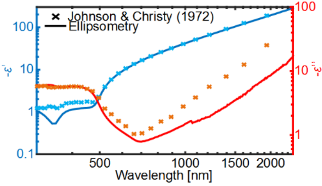
Fig. 3 Real and imaginary permittivity values of Au: Progress in fabrication has led to a reduction of plasmonic losses in noble metals by as much as a factor 2. The real ( \epsilon' ) and imaginary ( \epsilon'' ) parts of the permittivity are plotted as a function of the wavelength. The curves show the newly measured values (—solid lines) and the crosses (x) show the standard values as reported in Ref. [66], Image adapted from Ref. [43].
