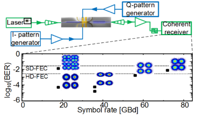
Fig. 15 IQ high-speed data transmission experiment: Laser light (green) is coupled to and from the chip by means of grating couplers, amplified and received coherently. The in- and quadrature phase components of the IQ modulator are encoded by electrical waveform generators (blue). The black squares indicate the received bit-error-ratios (BER) at some specific symbol rates. The corresponding constellation diagrams are plotted next to the squares. BER are below HD-FEC for symbol rates up to 54 GBd and below SD-FEC for QPSK at 72 GBd and 16-QAM 18 GBd resulting in line rates of 144 Gbit/s.
