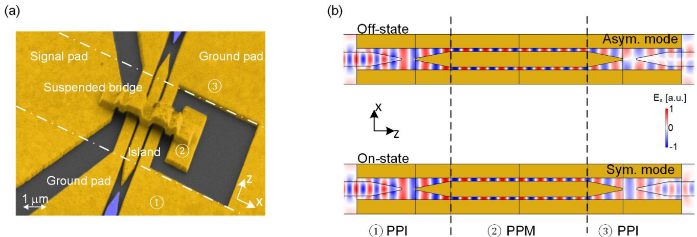
Fig. 8 The all-plasmonic MZM: (a) Colorized SEM image of the modulator. The plasmonic interferometer is formed by the metallic island and the metallic contact pads. An electrical signal can be applied to the island via a suspended bridge. Light is coupled to and from the interferometer by plasmonic-photonic interferometers (PPI). (b) FEM-simulations showing the plasmonic modes in the “off-” and “on-state”. In the off-state the fields are out of phase at the output, while they are in phase in the on-state. Light is coupled to guided modes of the silicon waveguide only when the modulator is in the “on-state”. Image adapted from Ref. [43].
