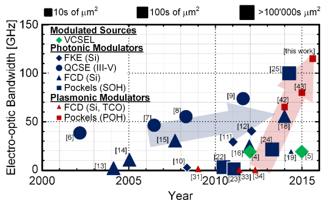
Fig. 1 Bandwidth and footprint of electro-optical integrated modulators (experimental results only) – The plot shows the improvement of the bandwidth over the last 15 years for integrated photonic and plasmonic modulator as well as directly modulated VCSELs. The size of the symbol indicates the required footprint and the shape of the symbol indicates the effect it relays on. It can be seen that photonic modulators have experienced a steady but moderate increase in bandwidth over the years (blue arrow). The plot also shows how newer plasmonic modulators are about to outperform the photonic counterparts at a much smaller footprint (red arrow). The expected bandwidth is well beyond 100s of GHz.
