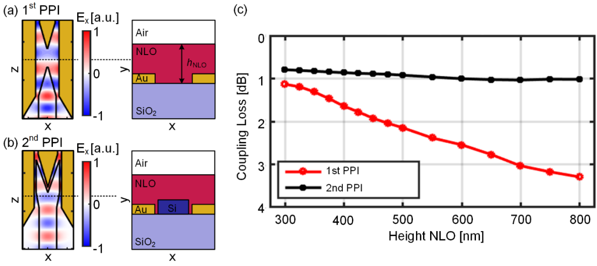
Fig. 11 Coupling schemas for conversion of light from a silicon waveguide to a slot SPP: (a) Shows the geometry of the coupler used in the initial proof of principle demonstration [43], while (b) shows the geometry of the improved coupling scheme as introduced in this and more recently in Ref. [44]. The blue/red fields show simulated field distributions. (c) Coupling losses as a function of the cladding height. The coupling efficiency of the old design in (a) strongly varies with the cladding height, while the new scheme from (b) is almost independent of the cladding height with coupling losses below 1 dB.
