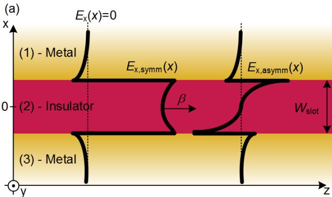
Fig. 4 Properties of plasmonic modes: (a) MIM-stack homogenous along y direction. Red indicates the insulating organic NLO material while yellow represents Au. The E_x field of the fundamental symmetric plasmonic mode is drawn in black. The field in the dielectric is quite enhanced over the field in the metal due to the large mismatch between NLO's and metals' permittivity. (b) Dispersion relation \beta(\omega) for frequencies ranging from 180 THz to 600 THz for the symmetric (solid line) and asymmetric (dashed) plasmonic modes at different slot widths. In the same plot we also give the dispersion relation of an uncoupled SPP as it would exist at a single MI interface. The gray area highlights all possible wave vectors of a hypothetical ideal photonic waveguide with an air-cladding and the nonlinear optical material as a guiding layer. Plasmonic modes are guided when their propagation constants \beta is larger than the NLO's light line. These modes are confined to the nearfield and cannot couple to photonic modes. The symmetric mode exists for all frequencies and widths while the asymmetric mode is cut-off for small frequencies and widths.
