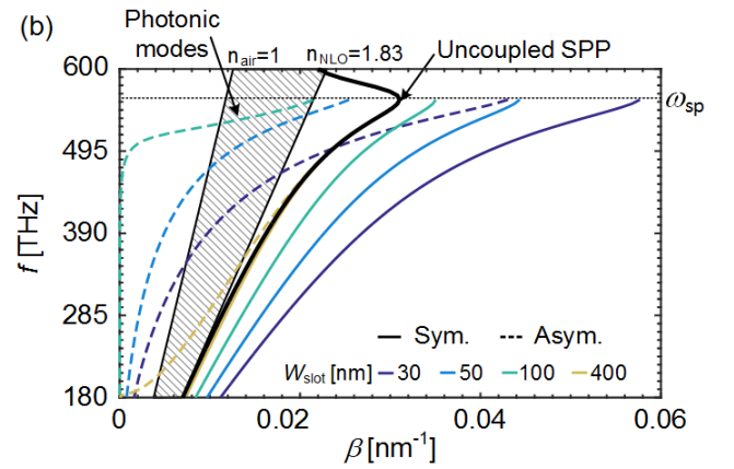
Fig. 4 Properties of plasmonic modes: (a) MIM-stack homogenous along y direction. Red indicates the insulating organic NLO material while yellow represents Au. The E_x field of the fundamental symmetric plasmonic mode is drawn in black. The field in the dielectric is quite enhanced over the field in the metal due to the large mismatch between NLO's and metals' permittivity. (b) Dispersion relation \beta(\omega) for frequencies ranging from 180 THz to 600 THz for the symmetric (solid line) and asymmetric (dashed) plasmonic modes at different slot widths. In the same plot we also give the dispersion relation of an uncoupled SPP as it would exist at a single MI interface. The gray area highlights all possible wave vectors of a hypothetical ideal photonic waveguide with an air-cladding and the nonlinear optical material as a guiding layer. Plasmonic modes are guided when their propagation constants \beta is larger than the NLO's light line. These modes are confined to the nearfield and cannot couple to photonic modes. The symmetric mode exists for all frequencies and widths while the asymmetric mode is cut-off for small frequencies and widths.
