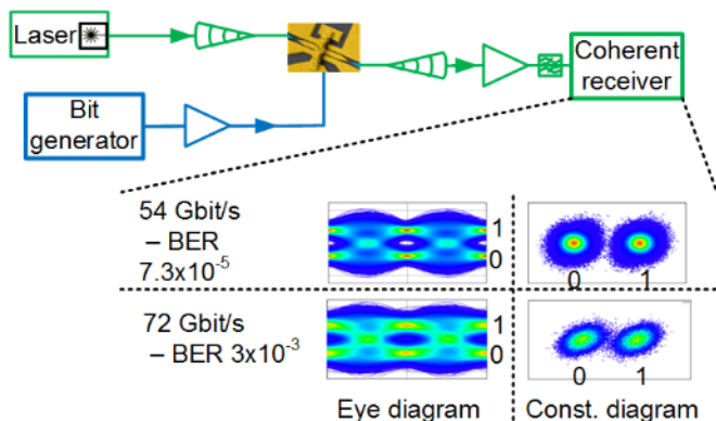
Fig. 13 MZM high-speed data transmission experiment: Laser light (green) is coupled to and from the chip by grating couplers, amplified and received coherently. The electrical signal (blue) generated by a bit generator is encoded by means of the modulator onto the optical carrier. The received eye diagram and constellation diagrams are shown at the bottom. The bit error ratios (BER) found with this device allow for high-speed data transmission up to 72 GB when utilizing hard decision forward error correction. (Image adapted from Ref. [43].)
