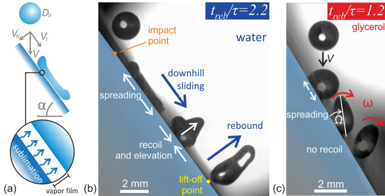
FIG. 1. Drop impact onto a tilted carbon dioxide sublimating surface: (a) schematic and image sequence of (b) water and (c) glycerol drop impacts. The impact conditions are \alpha = 55^\circ , We = \rho V^2 D_0 / \sigma = 86 , and Oh = \mu / \sqrt{\rho \sigma D_0} = 2.7 \times 10^{-3} for water and \alpha = 60^\circ , We = 121 , and Oh = 3.2 for glycerol. The image sequence was obtained by overlapping four images; see videos 1 and 2 in the SM [30] for the full sequence. The nondimensional rebound time is t_{reb}/\tau = 2.2 for water and t_{reb}/\tau = 1.2 for glycerol. Also indicated are the normal V_N and tangential V_T components of impact velocity, as well as the substrate tilt angle \alpha .
