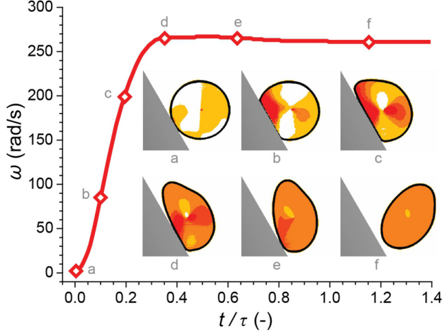
FIG. 7. History of the average angular velocity \omega of highly viscous liquid drop with Oh = 3.2 , We = 121 , and \alpha = 60^\circ during tumbling (simulation). Propagation of the dominant angular velocity component of \vec{\omega}_{loc} inside the drop is shown in the insets (a–f), at different stages of tumbling: stages a–c show the initial rise of the angular velocity shortly after the impact and stages d–f show rotation of the drop acting essentially as a solid. The drop rebounds (stage f) at t/\tau = 1.15 . A shading or color increase corresponds to the increase of the clockwise rotation.
