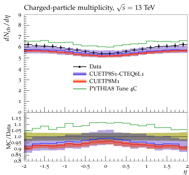
Fig. 22 CMS data at \sqrt{s} = 13 TeV [53] for the charged-particle pseudorapidity distribution, dN_{ch}/d\eta , in inelastic proton–proton collisions. The data are compared to predictions of PYTHIA8 using CUETP8S1-CTEQ6L1, CUETP8M1, and Tune 4C. The predictions based on CUETP8S1-CTEQ6L1 and CUETP8M1 are shown with an error band corresponding to the total uncertainty obtained from the eigentunes. Also shown are the ratios of these predictions to the data. The green band represents the total experimental uncertainty on the data
