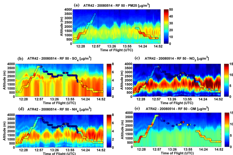
Figure 8. Vertical profiles (shadow) along the flight track of 14 May (RF50) of modelled \text{PM}_{2.5} (a), \text{SO}_4 (b), \text{NO}_3 (c), \text{NH}_4 (d), and OM (e). The circles are the measurements collected aboard the ATR42.
