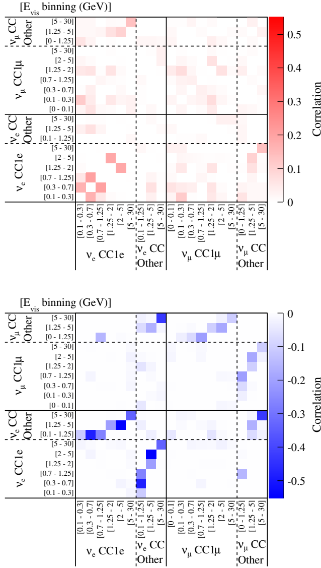
FIG. 24 (color online). The correlations between the estimated efficiencies for the final state topologies CC 1e and CC e other for the \nu_e CC event selection and CC 1 \mu and CC \mu other for the \nu_\mu CC event selection. The upper figure shows the combinations with positive correlation, and the lower with negative correlation. The diagonal correlations (correlation = 1) are not shown.
