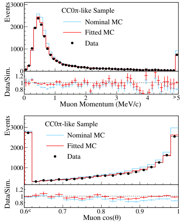
FIG. 14 (color online). Comparison of the data and Monte Carlo distributions for muon momentum (top) and angle (bottom) in the CC0 \pi -like sample, using the nominal and fitted values for the systematic parameters.
