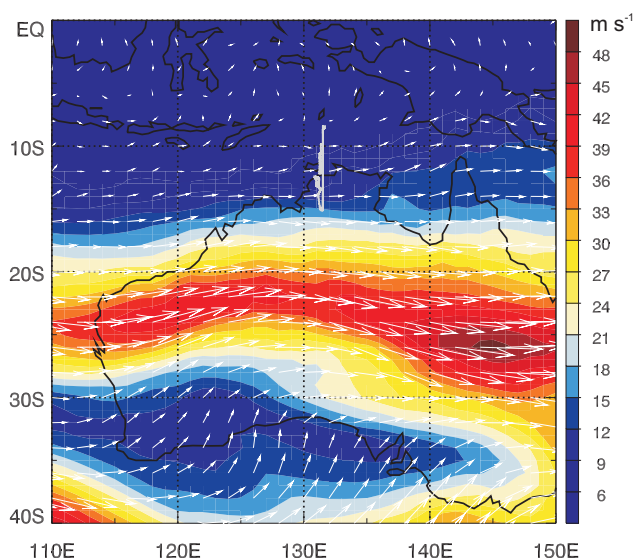
Fig. 6. ECMWF analysis for the wind velocity (in colour) and direction (white arrows) at the 200 hPa level ( \sim 12 km, anvil outflow) for 19 November 2005 at 06:00 UTC. The Falcon flight track over northern Australia is indicated in white.
