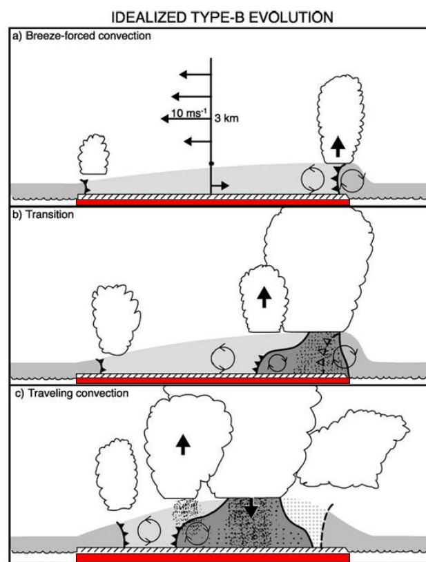
Fig. 2. Schematics of an idealised Hector type B evolution over the Tiwi Islands (red) in E–W cross section during the different development stages (a–c). In addition in (a) the typical westerly surface flow and easterly shear above is shown. Grey shaded areas indicate BLs and cold pools where the darkness is suggestive of coolness and precipitation is speckled. The hatched area to the rear of the mature cold pool in (c) is a recovering island BL after the convective interception of the original sea breeze front. The schematics are not according to scale (adapted from Carbone et al., 2000).
