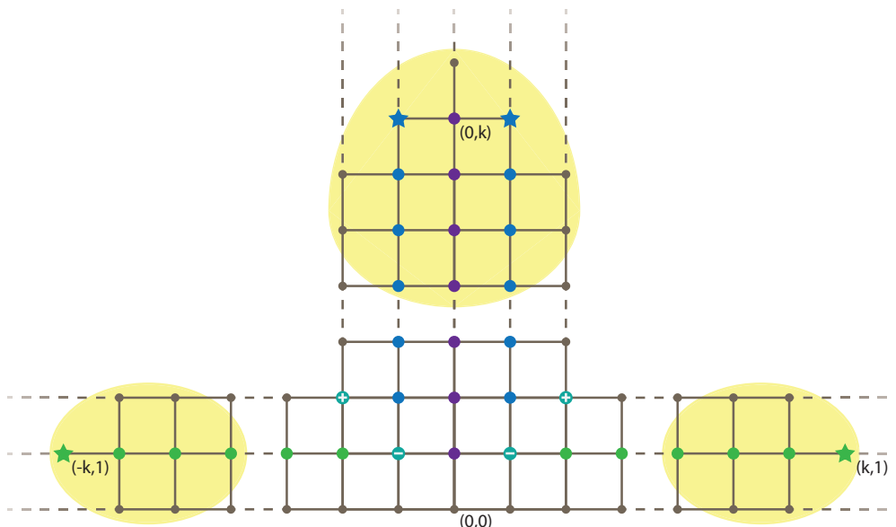
Figure 3. The T-hook lattice for T-functions satisfying the Hirota equations. There is a T-function T_{a,s} indicated by a gray dot at any lattice site (s, a) . The bigger coloured dots cover underlying gray dots and signify the Y-functions constructed out of nearest neighbour T-functions; the stars denote the special Y-functions which have no direct construction in terms of standard T-functions. By eliminating the special Y-functions, the consistency of the Y-system near the boundary is equivalent to a set of non-standard additional relations between the T-functions in each respective yellow bubble. These relations allow us to consider a truncation of the in principle infinite lattice of T-functions satisfying the Hirota equations.
