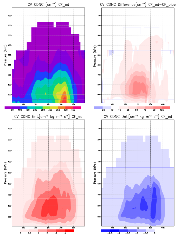
Fig. 3. The zonal and annual mean convective (CV) cloud droplet number concentration (CDNC) for the simulation CF ed , and CV CDNC difference between the two limiting cases (CF ed and CF pipe ) (top panels). The contribution of activated entrained aerosols to zonal and annual mean CV CDNC, and the reduction in the CV CDNC due to detrainment (bottom panels) (both multiplied by the vertical mass flux) for the simulation CF ed . Simulations are described in Table 2.
