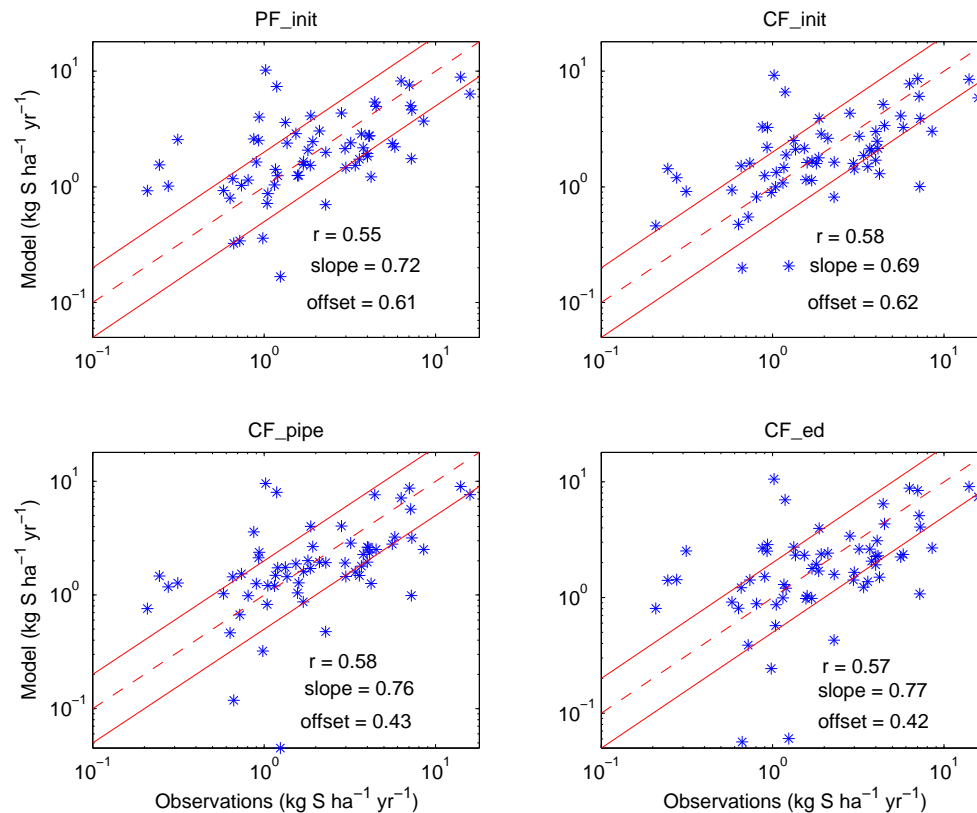
Fig. 8. Scatterplot of the observed and modeled wet deposition of sulfate from the dataset of Dentener et al. (2006a) (between 30° S and 30° N only) for the four simulations as described in Table 2.
