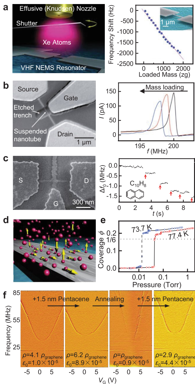
Figure 11.1. Mass sensing applications using NEMS resonators. (a) Schematic illustration of Xe atom mass sensing using a SiC NW resonator and the measured frequency response to mass loading, showing zg-level mass sensing. Reprinted in part with permission from ref 247. Copyright 2011 American Chemical Society. (b) SEM image and resonance curve during adsorption for a CNT resonator. Reprinted in part with permission from ref 71. Copyright 2008 American Chemical Society. (c) SEM image and mass sensing data for a CNT resonator, showing down to 1.7 yoctogram resolution. Reprinted in part with permission from ref 250. Copyright 2012 Nature Publishing Group. (d) Schematic illustration of fluctuation of Xe atoms (including adsorption, desorption, and surface diffusion) on a SiC NW resonator. Reprinted in part with permission from ref 247. Copyright 2011 American Chemical Society. (e) Low-dimensional phase transition of Kr atoms adsorbed on the surface of a CNT resonator, detected by monitoring the resonance frequency. Reprinted in part with permission from ref 42. Copyright 2010 American Association for the Advancement of Science. (f) Mass sensing behavior of graphene resonator. Reprinted in part with permission from ref 57. Copyright 2009 Nature Publishing Group.
