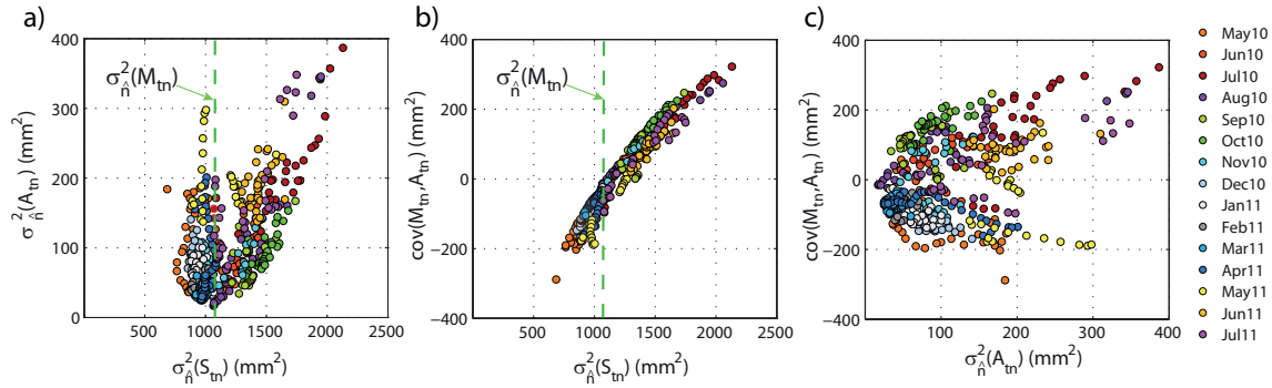
Fig. 6. Scatter plots of (a) the spatial variance of absolute soil moisture ( \sigma_{\bar{n}}^2(S_{tn}) ) vs. spatial variance of anomalies ( \sigma_{\bar{n}}^2(A_{tn}) ), (b) spatial variance of absolute soil moisture vs. spatial covariance of temporal mean and anomalies 2 \cdot \text{cov}(M_{tn}, A_{tn}) , and of (c) spatial variance of anomalies vs. the spatial covariance between the mean and anomalies. The green dotted line represents the variance of spatial temporal mean ( \sigma_{\bar{n}}^2(M_{tn}) ).
