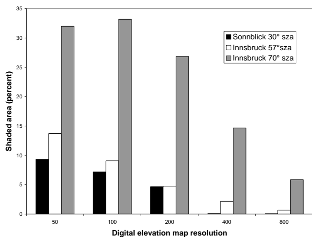
Fig. 4. Overview of the shaded areas as a function of the digital elevation map resolution. The simulations were performed using the digital elevation maps of the Innsbruck and Sonnblick regions. For the “Innsbruck” simulations, solar zenith angles of 57 and 70 degree were used and for the “Sonnblick” simulations a solar zenith angle of 30 degrees was used.
