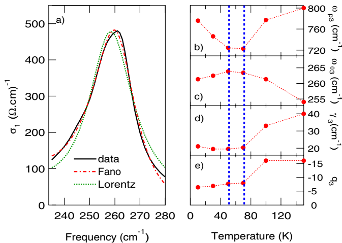
Fig. 5. (Color online) (a) Blow-up of \sigma_1(\omega) around the mode at 261 \text{ cm}^{-1} at 10 K and for E \perp b . The fits of this mode with either a Lorentz harmonic oscillator or a Fano lineshape are shown for comparison. (b) Temperature dependence of the oscillator strength \omega_{p3} , (c) resonance frequency \omega_{03} , (d) scattering rate \gamma_3 , and (e) asymmetry factor q_3 of the mode at 261 \text{ cm}^{-1} within the Fano-like fit. The blue dashed lines indicate the lower and upper limits of T_{MI}^{\perp b} , respectively.
