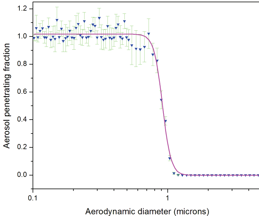
Fig. 3. Aerosol penetrating fraction of the impactor used. Note the sharp cut-off at 1\ \mu\text{m} aerodynamic diameter. The magenta curve is the sigmoid fit of the blue data points. Green error bars represent the standard deviation of the measurements.
