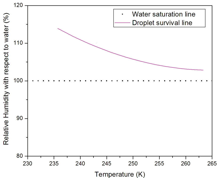
Fig. 2. Experimental determination of the water droplet survival line (water breakthrough) for different temperatures. Above the droplet survival line, the OPC can not distinguish ice crystals and water droplets.
