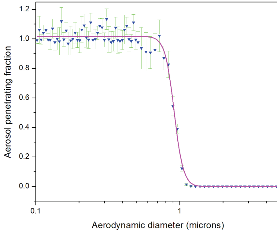
Fig. 3. Aerosol penetrating fraction of the impactor used. Note the sharp cut-off at 1\text{ }\mu\text{m} aerodynamic diameter. The magenta curve is the sigmoid fit of the blue data points. Green error bars represent the standard deviation of the measurements.
