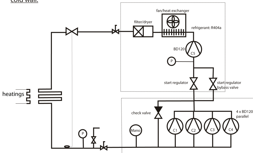
Fig. 1. Schematic of the cooling system in PINC.
