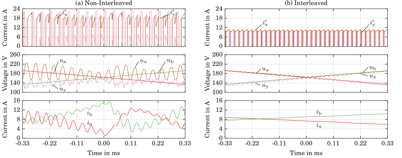
Fig. 3. Detailed simulation results of the first intersection of the mains line-to-neutral voltages u_a and u_b at \omega t \approx 60^\circ : (a) the discontinuous buck converter input currents i'_x , i'_y of the non-interleaved SWISS Rectifier lead to high switching frequency ripples of the input filter capacitor voltages u_x and u_y . As u_x and u_y cannot intersect due to D_{y\bar{p}} and S_{x\bar{p}} a distortion of the mains currents i_a and i_b results [12]. (b) In case of an interleaved SWISS Rectifier the amplitude of i'_x , i'_y is reduced and the frequency is doubled which leads to a significant reduction of the ripples in u_x and u_y .
