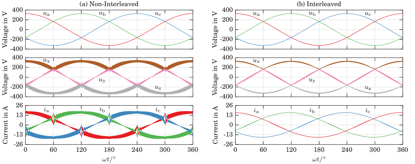
Fig. 2. Simulation results for an 8 kW SWISS Rectifier as specified in Table I , showing the ac input voltages u_{a,b,c} , the filter capacitor voltages u_{x,y,z} and the resulting ac input currents i_{a,b,c} . (a) Due to the discontinuous input currents i'_{x,y,z} of the non-interleaved dc-dc buck converters a high ripple in u_{x,y,z} and in the ac input currents i_{a,b,c} results. This also leads to significant distortions in i_{a,b,c} as described in [12]. (b) In the interleaved SWISS Rectifier the switching frequency voltage ripples of u_{x,y,z} are reduced significantly due to harmonic cancellation. Therefore the ac input current ( i_{a,b,c} ) ripple and the resulting distortion at sector boundaries are reduced as well.
