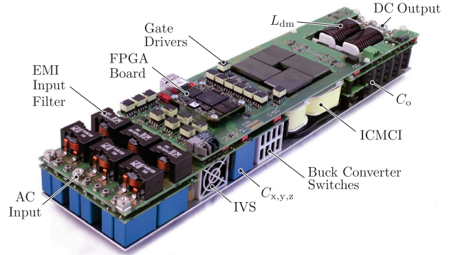
Fig. 9. Implemented 8 kW 400 V ac / 400 V dc interleaved SWISS Rectifier prototype ( 420 \text{ mm} \times 95 \text{ mm} \times 50 \text{ mm} ) with > 99\% efficiency (cf. Fig. 11 ) and a power density of 4 \text{ kW dm}^{-3} ( 66 \text{ W in}^{-3} ).
