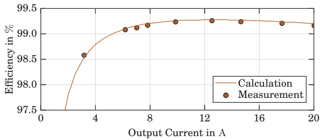
Fig. 11. Calculated and measured efficiency of the rectifier as function of I_1 , indicating that the converter achieves an efficiency above 99% for > 30% load with peak efficiency of 99.26%. Measurements were taken on the prototype shown in Fig. 9 using a Yokogawa WT3000 power analyzer.
