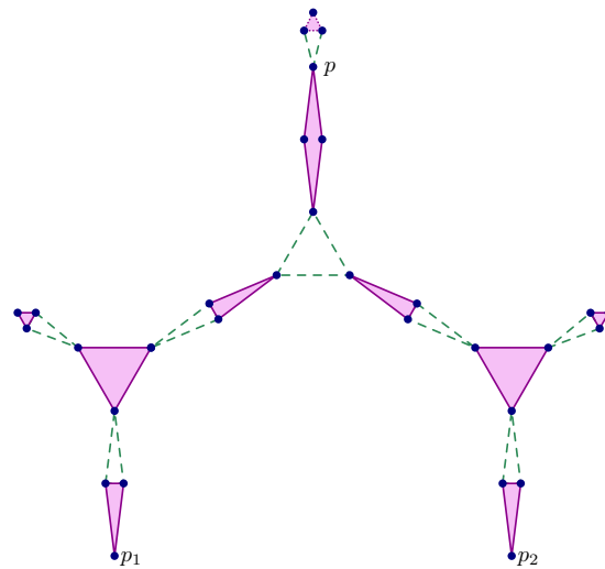
Figure 5: Split gadget: points p , p_1 , and p_2 are covered by cycles of total length 18a + 10\epsilon .
