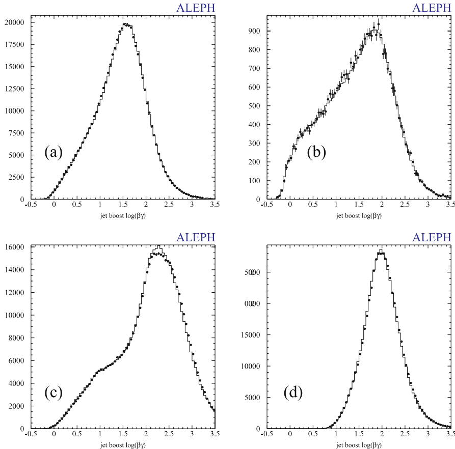
Fig. 9. Distributions of jet boosts ( \log \beta_{\text{jet}} \gamma_{\text{jet}} ) for data ( circles ) and MC ( histogram ): a from Z \rightarrow q\bar{q} events (1998–2000) and b from high energy di-jet events (183–209 GeV) using the Durham jet reconstruction in the standard analysis, c and d from Z \rightarrow q\bar{q} events using PCUT and CONE reconstructions respectively
