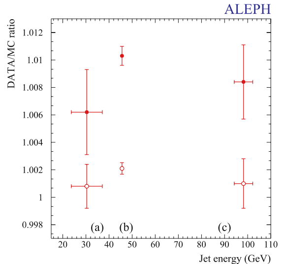
Fig. 2. Data/MC ratio of average E_{\text{jet}}/E_{\text{beam}} for E_{\text{jet}} energies of (a) 3-jet events at the Z , (b) di-jet events at the Z and (c) high energy di-jet events. Closed points : |\cos\theta_{\text{jet}}| > 0.7 , open points : |\cos\theta_{\text{jet}}| < 0.7
