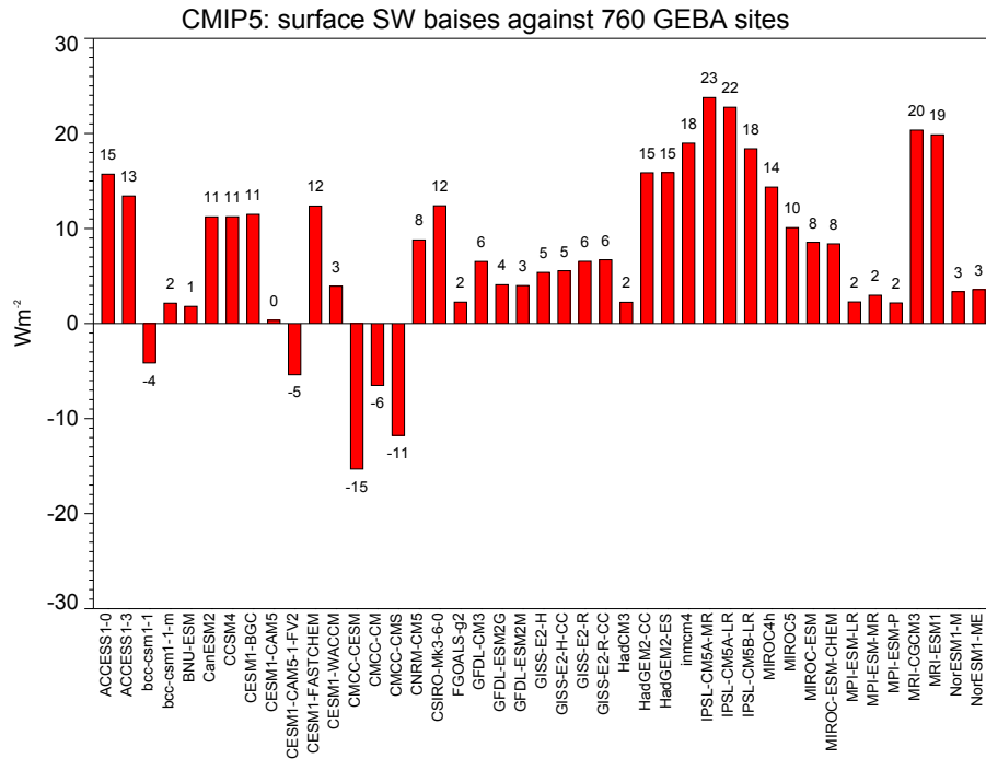
Figure 7. Average biases (model – GEBA observations) in surface downward shortwave radiation ( W m^{-2} ) at Earth’s surface calculated in 43 different CMIP5 climate models averaged over 760 sites from GEBA. Adapted from Wild et al., 2015.
