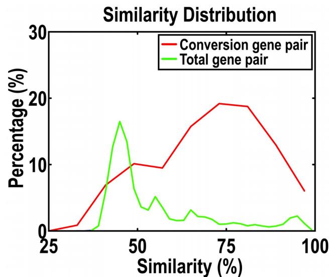
Figure 3 Gene conversions are favored between similar genes. Sequence similarities were calculated for homologs involved in gene conversions and for all homologs.
