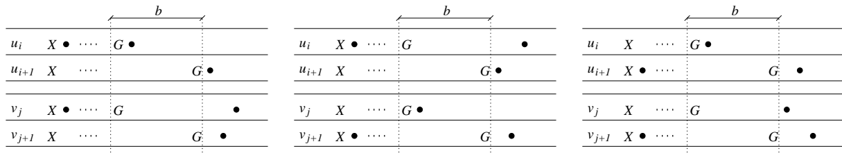
Figure 3: The edge gadget in three possible situations with the corresponding optimal schedule.
