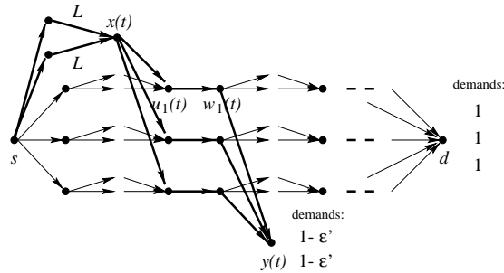
Figure 4: Construction enforcing that at most one flow path touches a column
