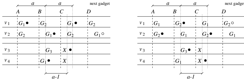
Figure 1: Two schedules which minimize the ART for the duplicator gadget. The dots mark which message is broadcast. The left situation corresponds to v being in the independent set, the right one to v not being in.
